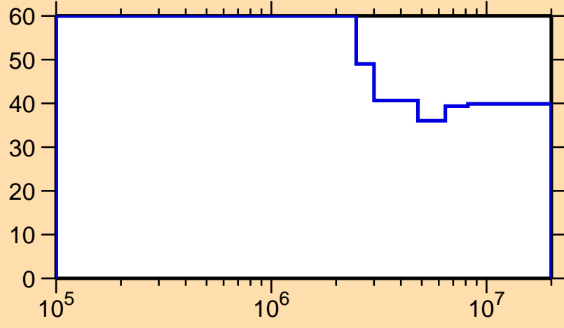
\Delta\sigma/\sigma vs. E for ^{126}\text{Pr}(n,n\text{cont.})
