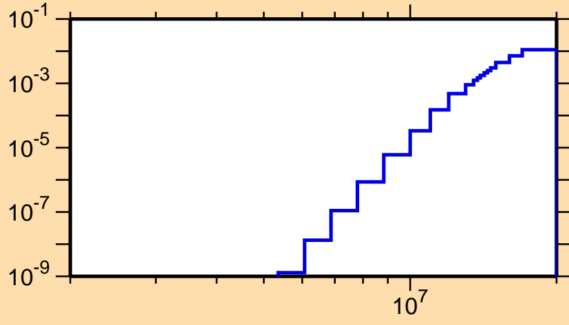
\sigma vs. E for ^{128}\text{Pr}(n,n\alpha)
