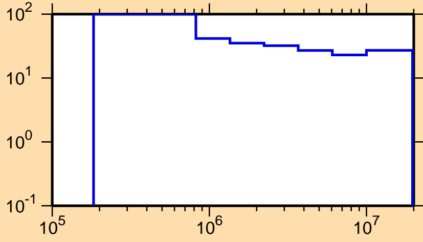
\Delta\sigma/\sigma vs. E for ^{128}\text{Pr}(n,n_1)
