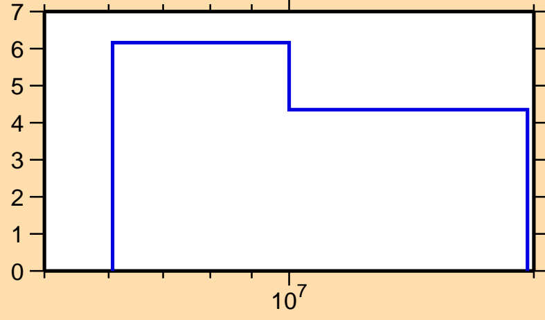
\Delta\sigma/\sigma vs. E for ^{128}\text{Pr}(n,\text{tot.})
