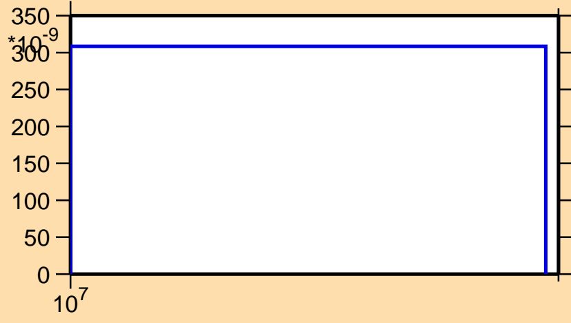
\sigma vs. E for ^{128}\text{Pr}(n,\text{pt})
