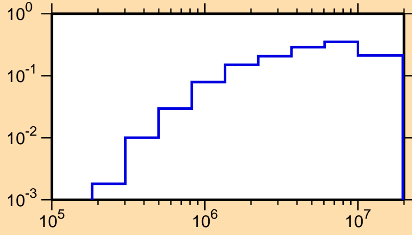
\sigma vs. E for ^{128}\text{Pr}(n,\text{inel.})
