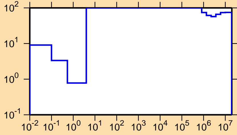
\Delta\sigma/\sigma vs. E for ^{128}\text{Pr}(n,\gamma)
