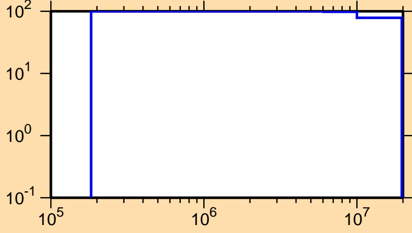
\Delta\sigma/\sigma vs. E for ^{128}\text{Pr}(n,n\text{cont.})
