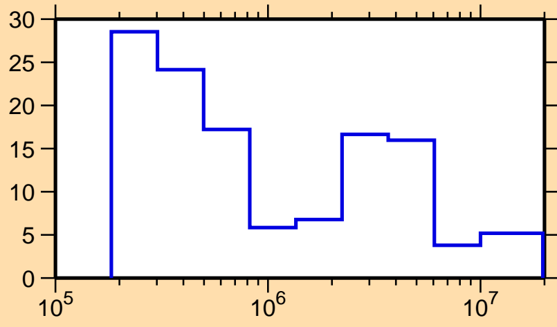
\Delta\sigma/\sigma vs. E for ^{128}\text{Pr}(n,\text{el.})
