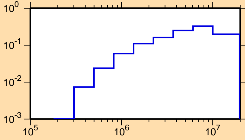
\sigma vs. E for ^{128}\text{Pr}(n,n\text{cont.})
