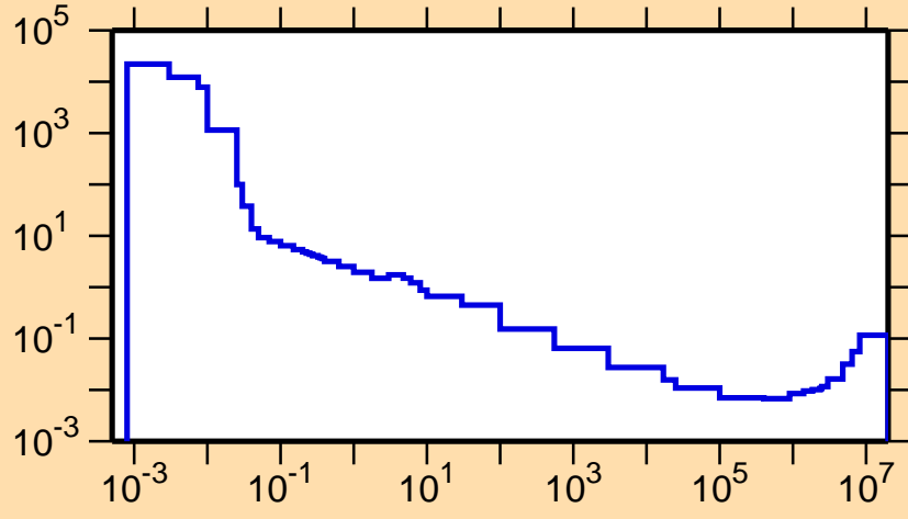
\sigma vs. E for ^{128}\text{Pr}(n,\alpha)
