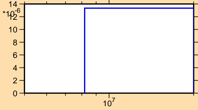
\sigma vs. E for ^{128}\text{Pr}(n,pd)
