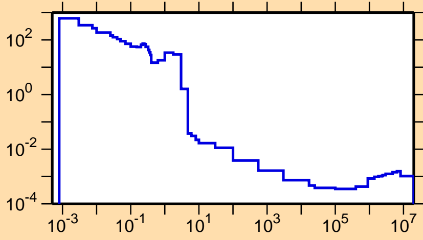
\sigma vs. E for ^{128}\text{Pr}(n,\gamma)
