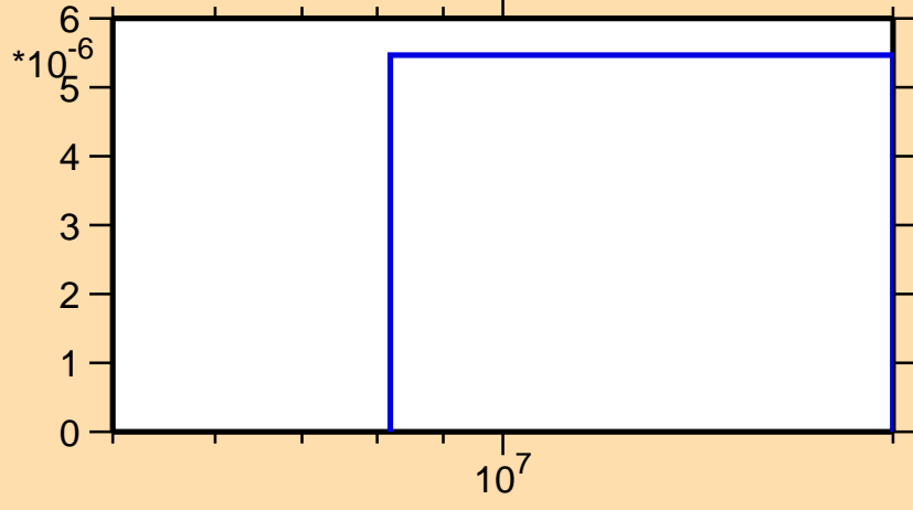
\sigma vs. E for ^{128}\text{Pr}(\text{mt } 45)
