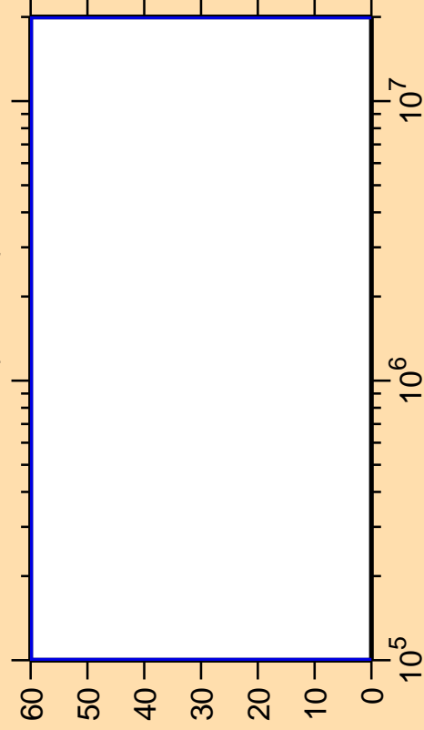
\Delta\sigma/\sigma vs. E for ^{128}\text{Pr}(n,\text{inel.})
