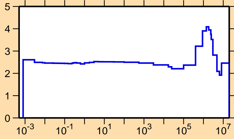
\sigma vs. E for ^{128}\text{Pr}(n,\text{el.})
