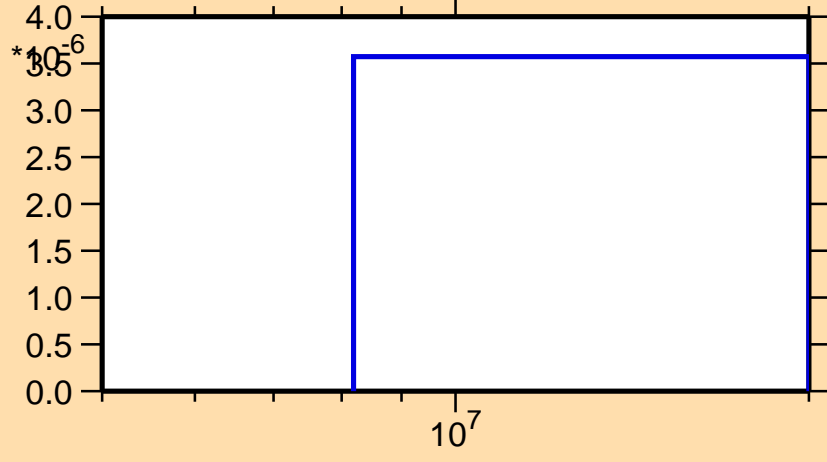
\sigma vs. E for ^{128}\text{Pr}(n,\text{nd})
