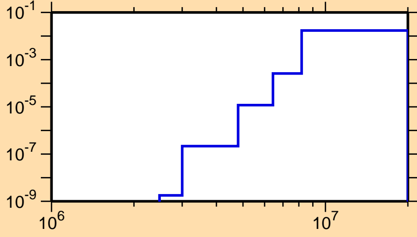
\sigma vs. E for ^{128}\text{Pr}(n,d)
