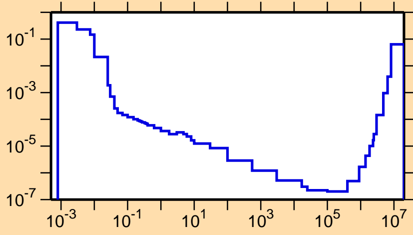
\sigma vs. E for ^{128}\text{Pr}(n,p\alpha)
