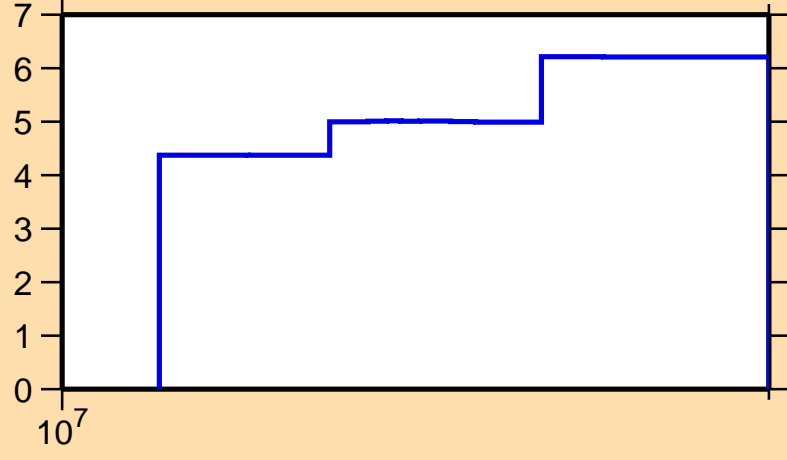
\Delta\sigma/\sigma vs. E for ^{129}\text{Pr}(n,\text{tot.})
