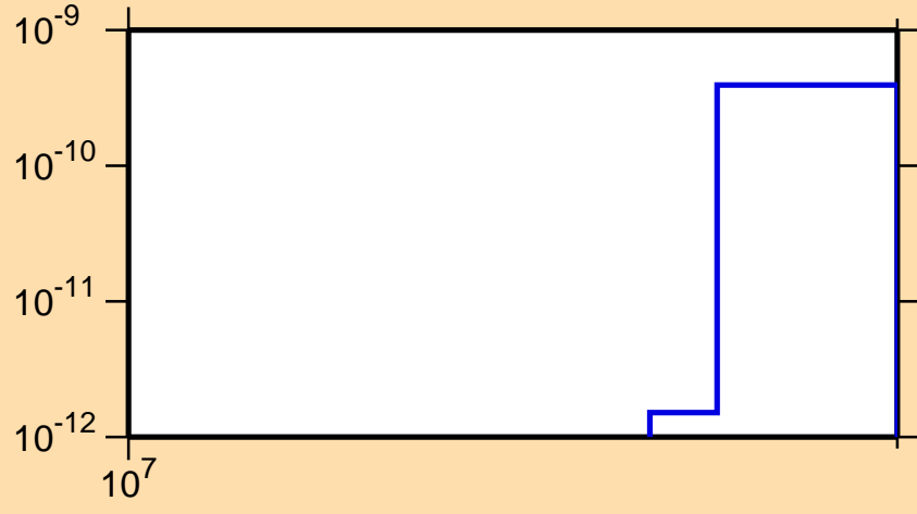
\sigma vs. E for ^{129}\text{Pr}(n,2n\alpha)
