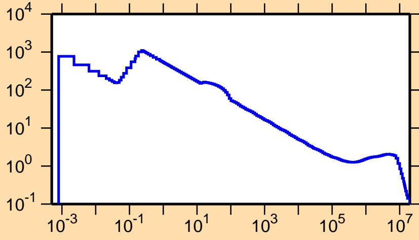
\sigma vs. E for ^{129}\text{Pr}(n,p)
