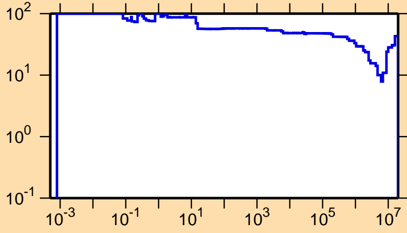
\Delta\sigma/\sigma vs. E for ^{129}\text{Pr}(n,p)
