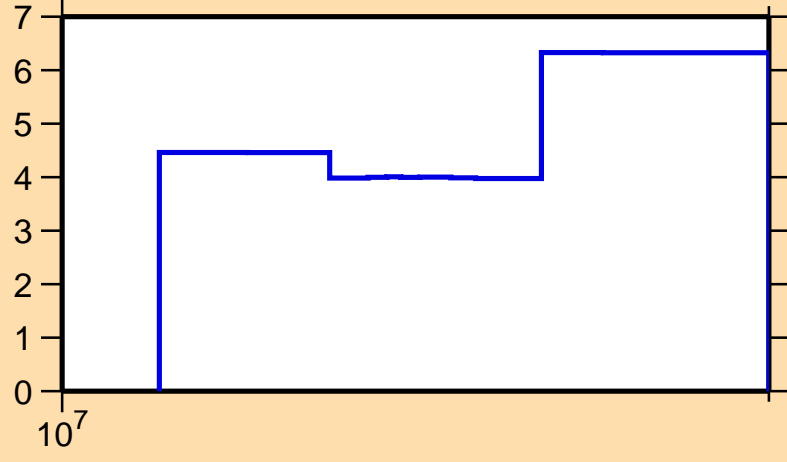
\Delta\sigma/\sigma vs. E for ^{129}\text{Pr}(n,\text{el.})
