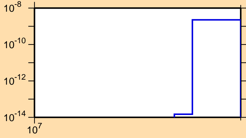
\sigma vs. E for ^{129}\text{Pr}(n,nt)
