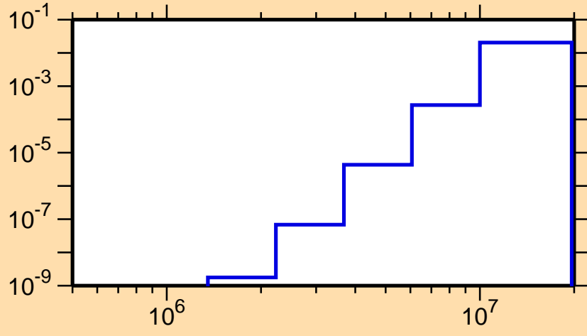
\sigma vs. E for ^{129}\text{Pr}(n,p\alpha)
