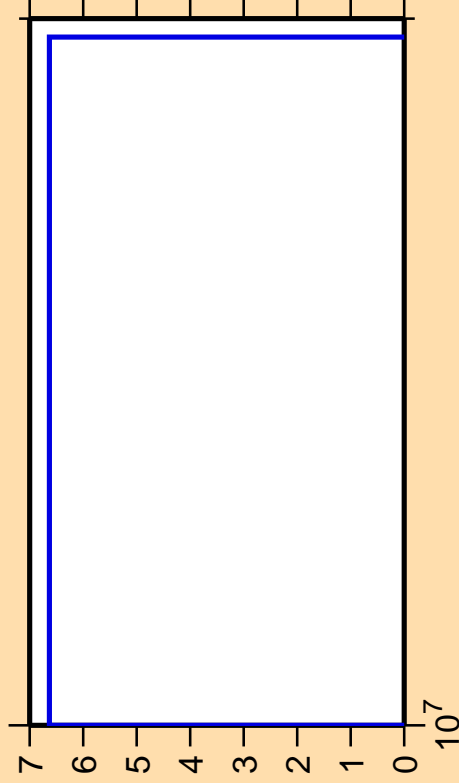
\Delta\sigma/\sigma vs. E for ^{129}\text{Pr}(\text{mt } 34)
