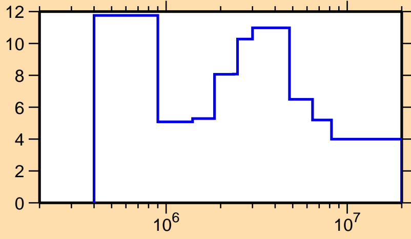
\Delta\sigma/\sigma vs. E for ^{129}\text{Pr}(n, el.)
