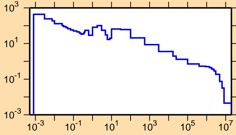
\sigma vs. E for ^{129}\text{Pr}(n,\gamma)
