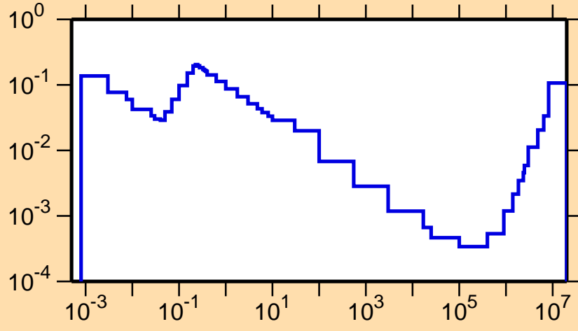
\sigma vs. E for ^{129}\text{Pr}(n,\alpha)
