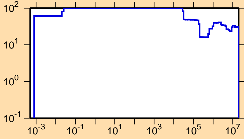
\Delta\sigma/\sigma vs. E for ^{130}\text{Pr}(n,p)
