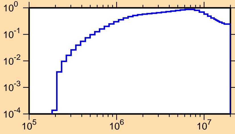
\sigma vs. E for ^{130}\text{Pr}(n,n\text{cont.})
