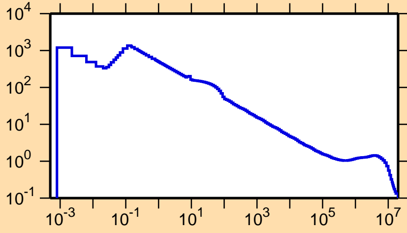
\sigma vs. E for ^{130}\text{Pr}(n,p)
