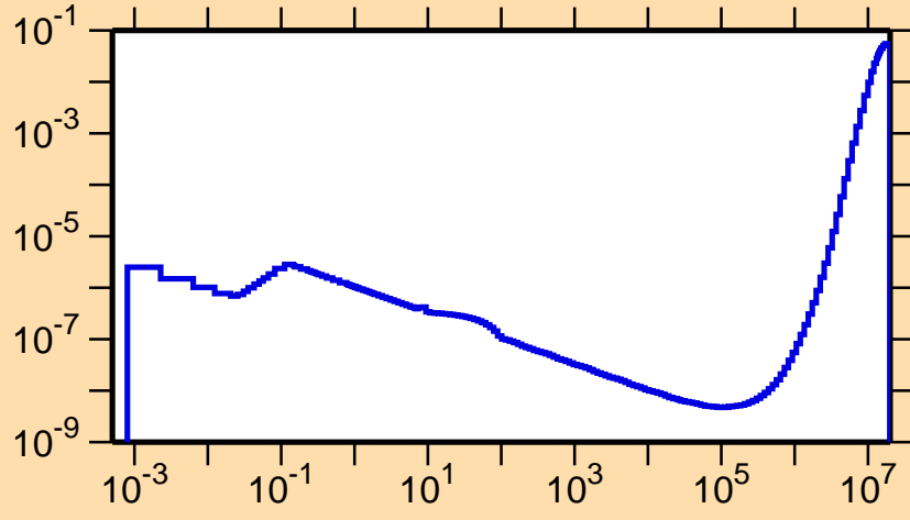
\sigma vs. E for ^{130}\text{Pr}(n,p\alpha)
