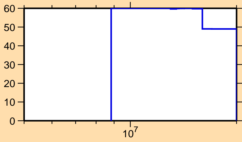
\Delta\sigma/\sigma vs. E for ^{130}\text{Pr}(n,2n)
