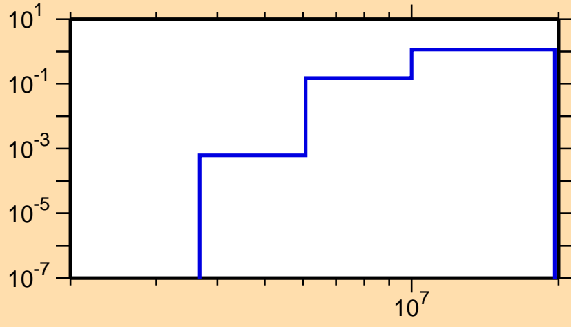
\sigma vs. E for ^{130}\text{Pr}(n,np)
