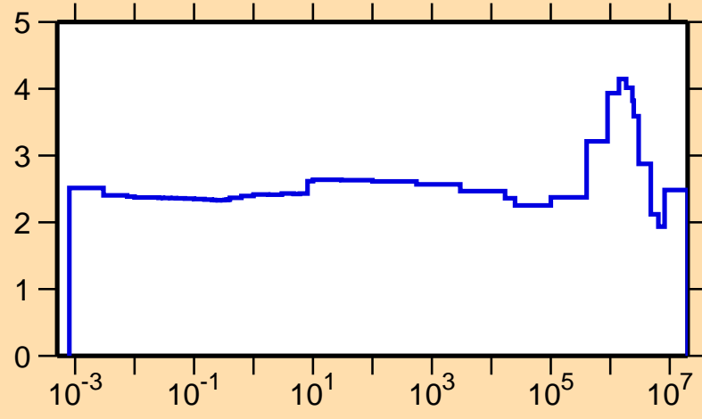
\sigma vs. E for ^{130}\text{Pr}(n,\text{el.})
