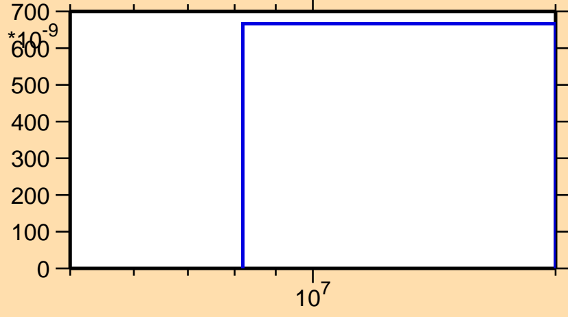
\sigma vs. E for ^{130}\text{Pr}(\text{mt } 45)
