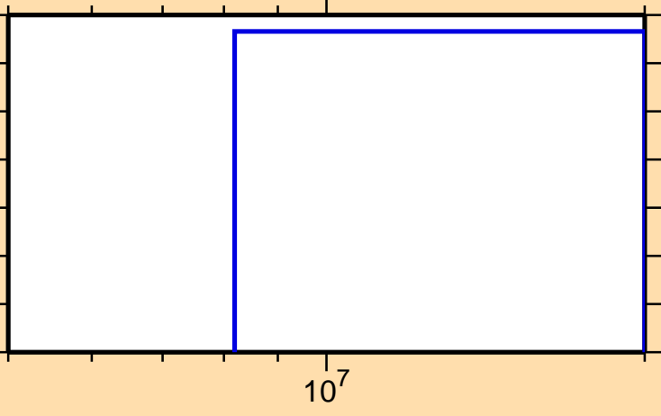
\sigma vs. E for ^{130}\text{Pr}(n,\text{nd})
