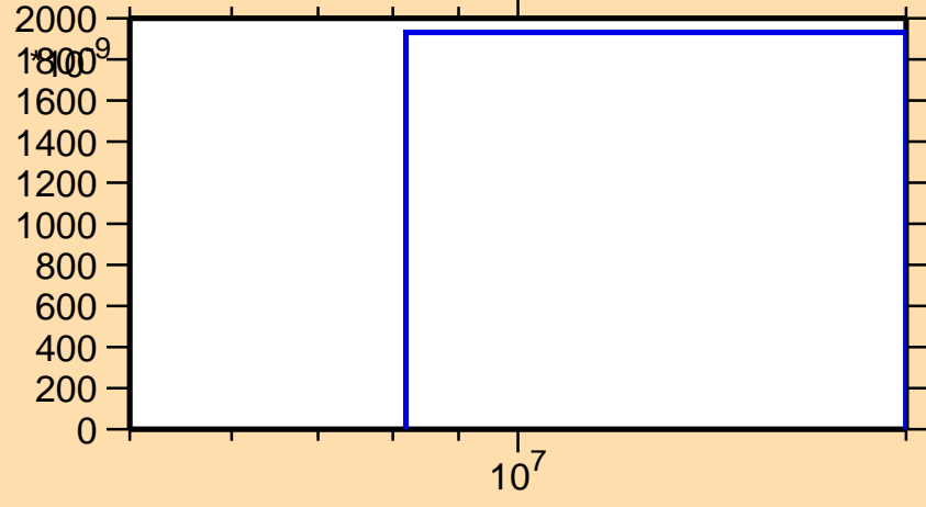
\sigma vs. E for ^{130}\text{Pr}(n,\text{pd})
