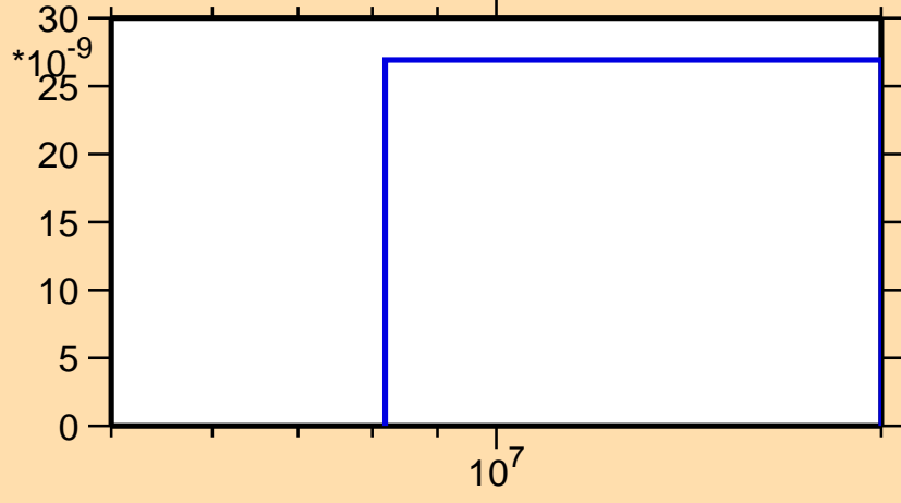
\sigma vs. E for ^{130}\text{Pr}(n,\text{pt})
