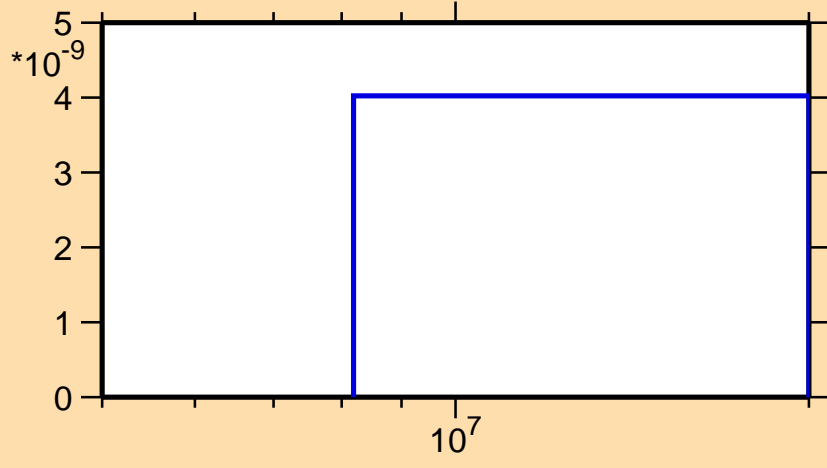
\sigma vs. E for ^{130}\text{Pr}(\text{mt117})
