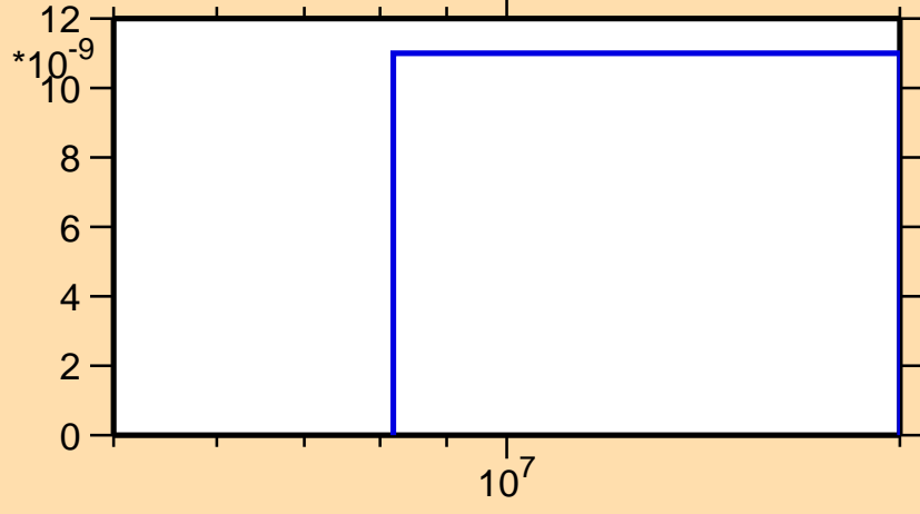
\sigma vs. E for ^{130}\text{Pr}(n,2n\alpha)
