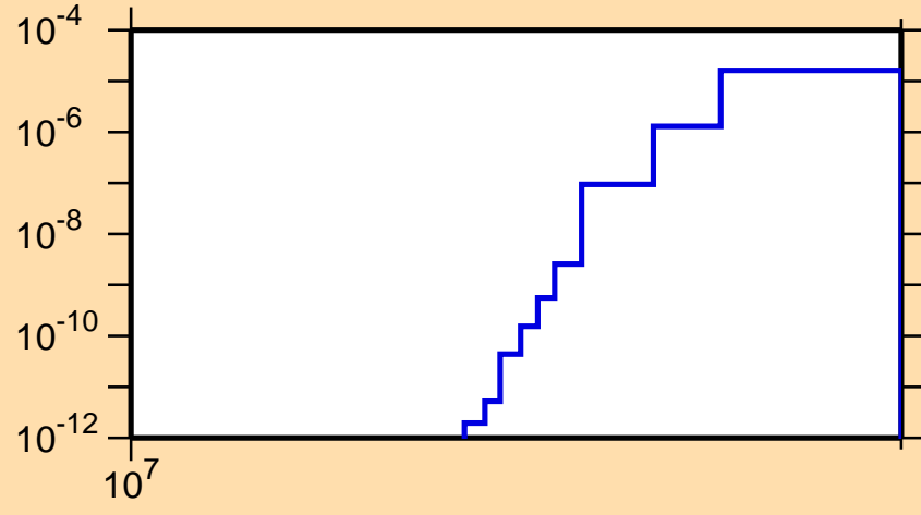
\sigma vs. E for ^{131}\text{Pr}(n,nd)
