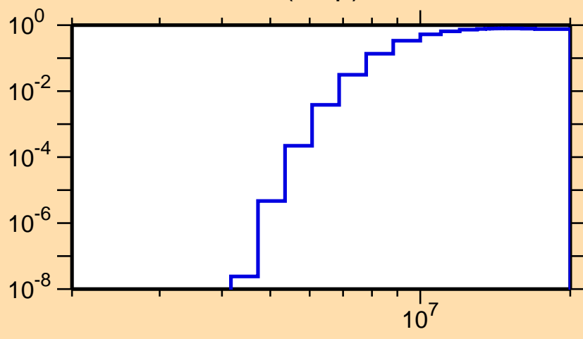
\sigma vs. E for ^{132}\text{Pr}(n,np)
