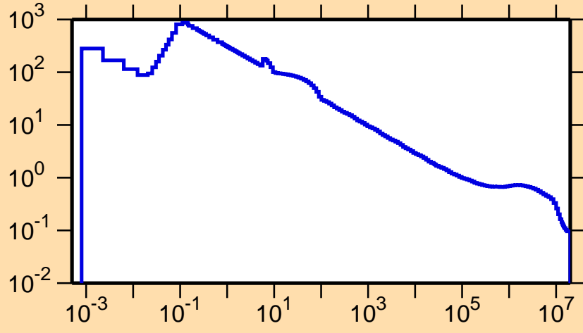
\sigma vs. E for ^{132}\text{Pr}(n,p)
