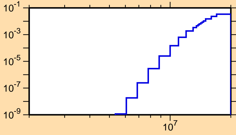
\sigma vs. E for ^{132}\text{Pr}(n,n\alpha)
