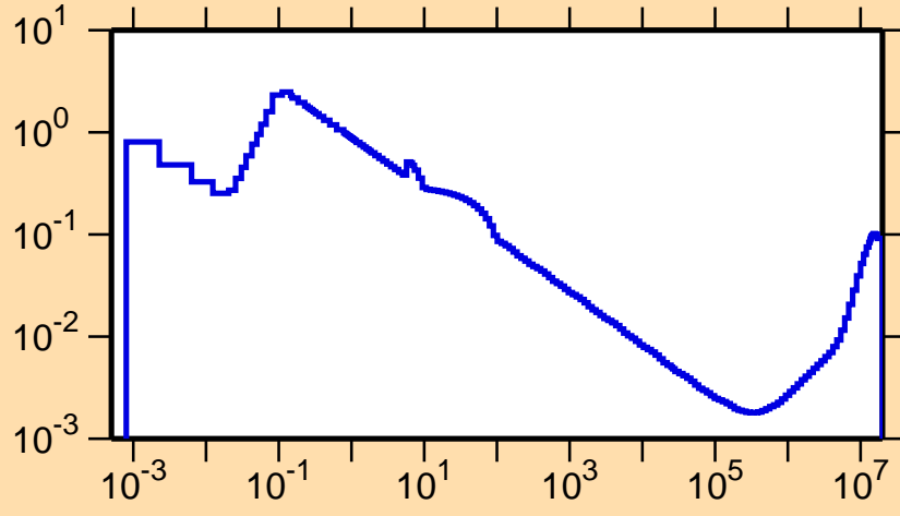
\sigma vs. E for ^{132}\text{Pr}(n,\alpha)
