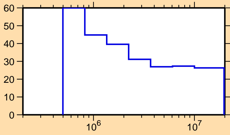
\Delta\sigma/\sigma vs. E for ^{132}\text{Pr}(n,n\text{cont.})
