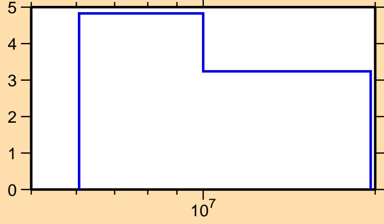
\Delta\sigma/\sigma vs. E for ^{132}\text{Pr}(n,\text{tot.})
