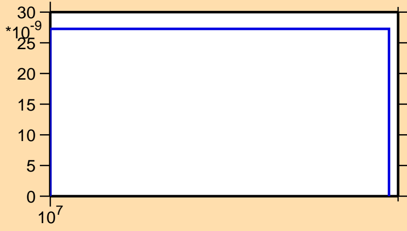
\sigma vs. E for ^{132}\text{Pr}(n,2n\alpha)
