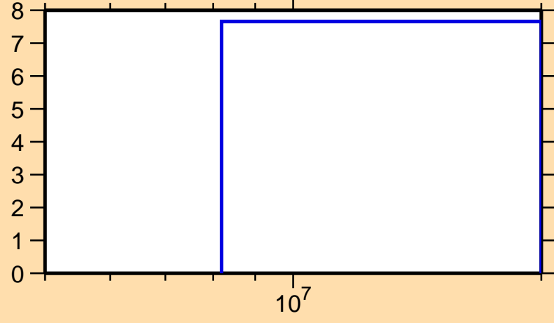
\Delta\sigma/\sigma vs. E for ^{132}\text{Pr}(n,\text{el.})
