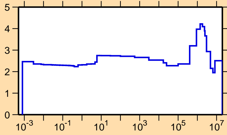
\sigma vs. E for ^{132}\text{Pr}(n,\text{el.})
