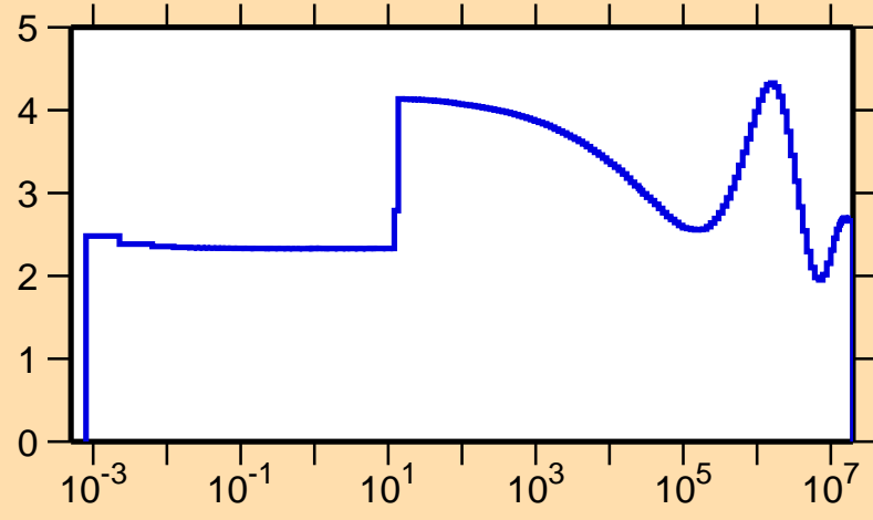
\sigma vs. E for ^{133}\text{Pr}(n,\text{el.})
