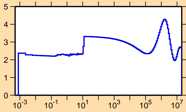
\sigma vs. E for ^{134}\text{Pr}(n,\text{el.})
