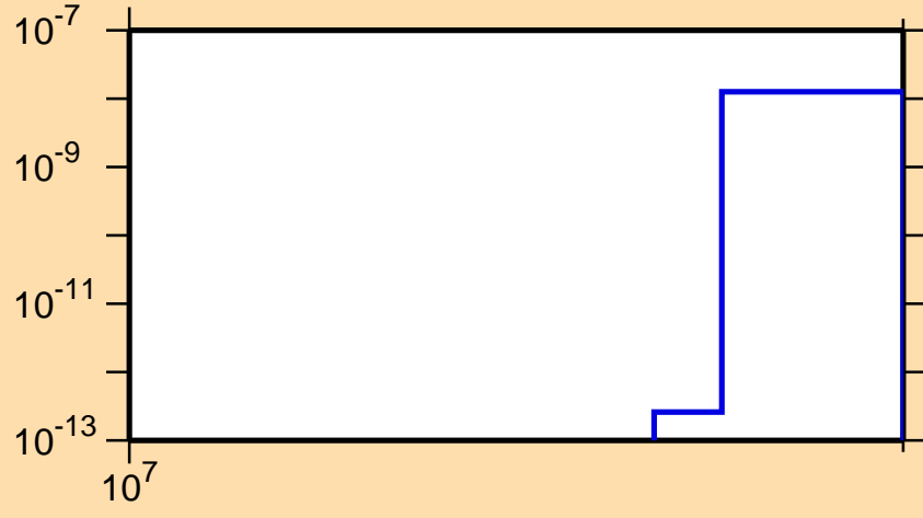
\sigma vs. E for ^{134}\text{Pr}(n,nt)
