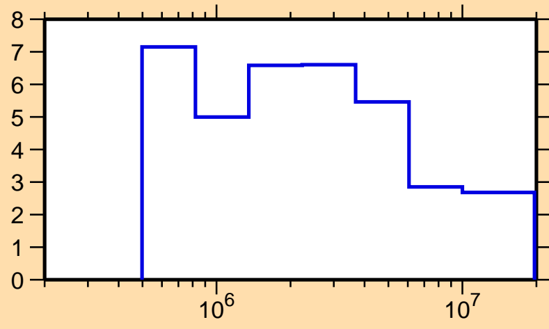
\Delta\sigma/\sigma vs. E for ^{134}\text{Pr}(n, \text{tot.})
