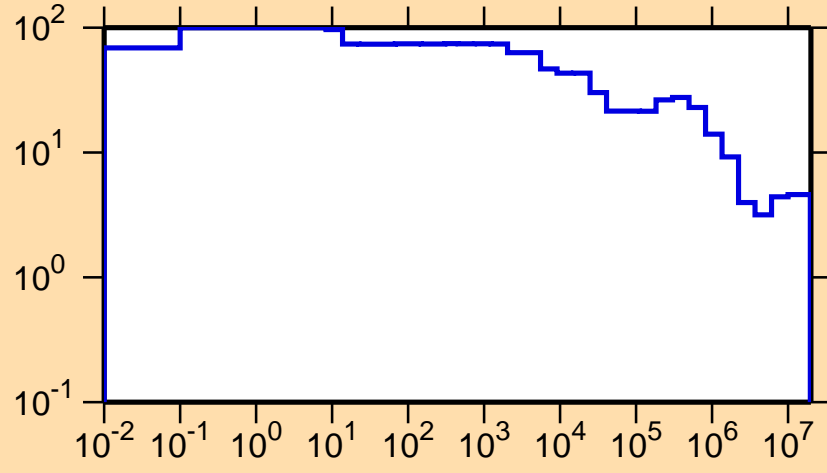
\Delta\sigma/\sigma vs. E for ^{134}\text{Pr}(n,\text{nonel.})
