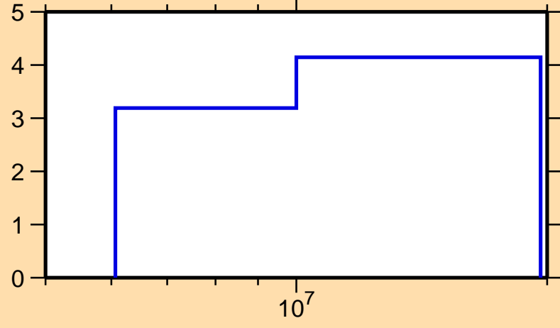
\Delta\sigma/\sigma vs. E for ^{134}\text{Pr}(n,\text{el.})
