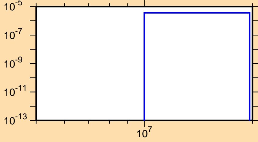
\sigma vs. E for ^{134}\text{Pr}(n,nd)
