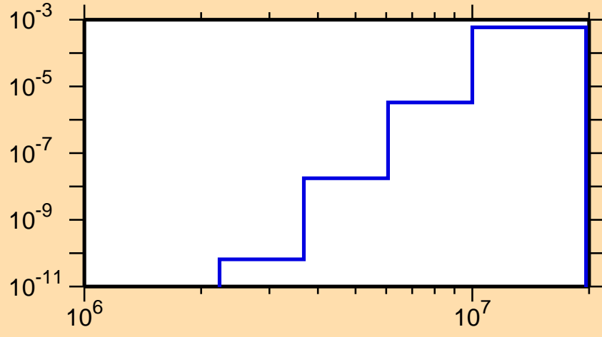
\sigma vs. E for ^{134}\text{Pr}(n,p\alpha)
