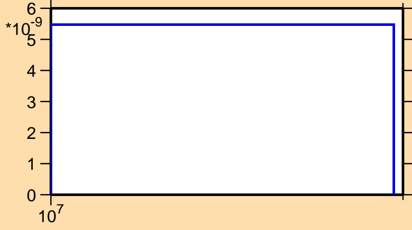
\sigma vs. E for ^{134}\text{Pr}(\text{mt } 45)
