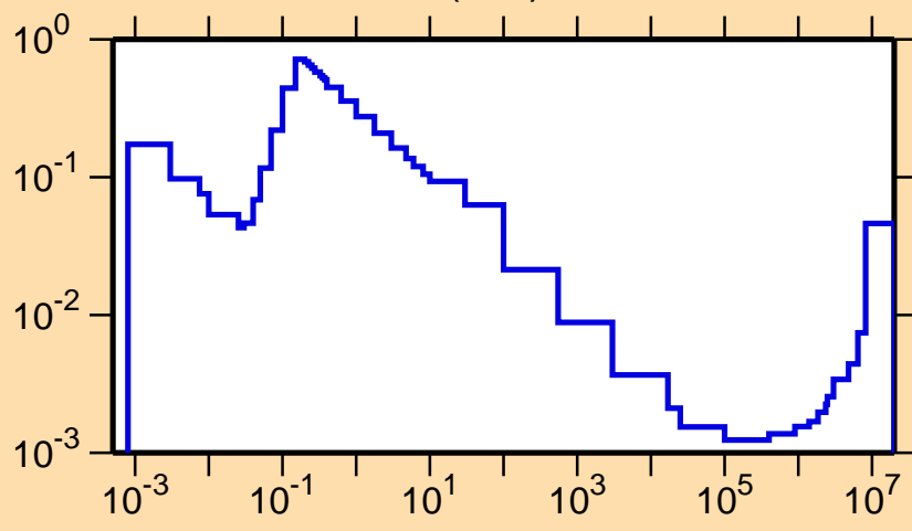
\sigma vs. E for ^{134}\text{Pr}(n,\alpha)
