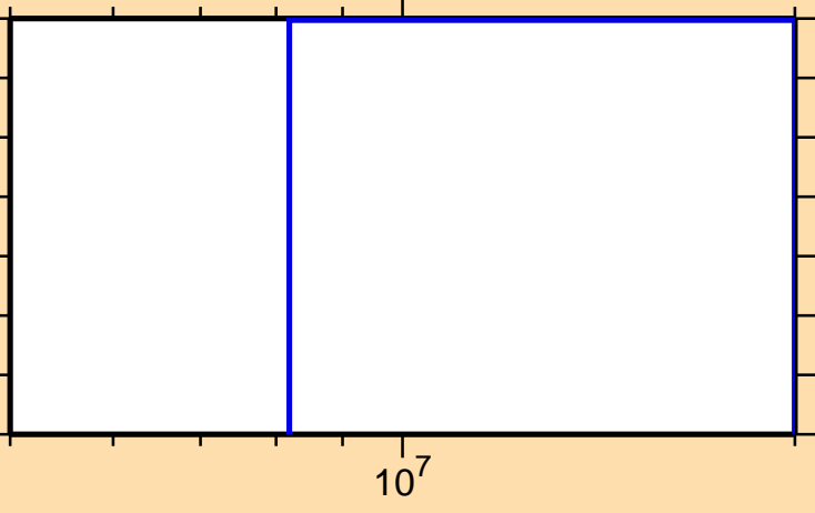
\sigma vs. E for ^{134}\text{Pr}(n,\text{pt})
