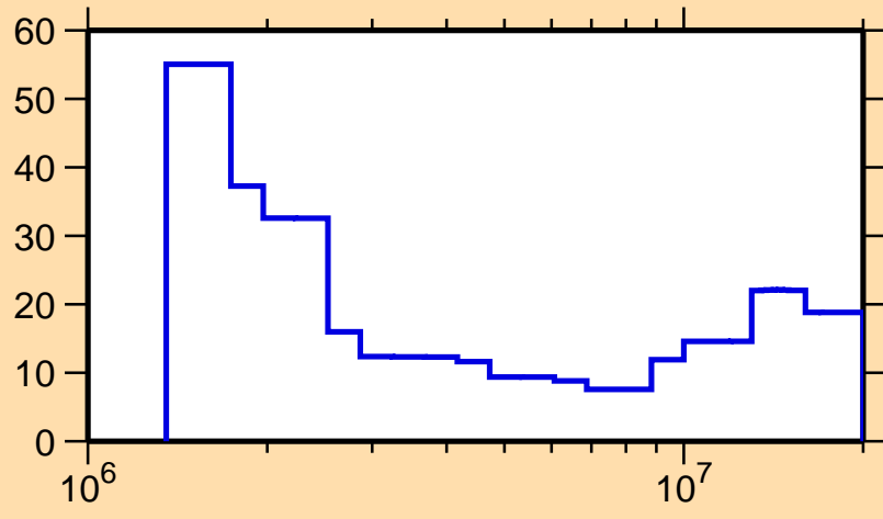
\Delta\sigma/\sigma vs. E for ^{135}\text{Pr}(n,n\text{cont.})
