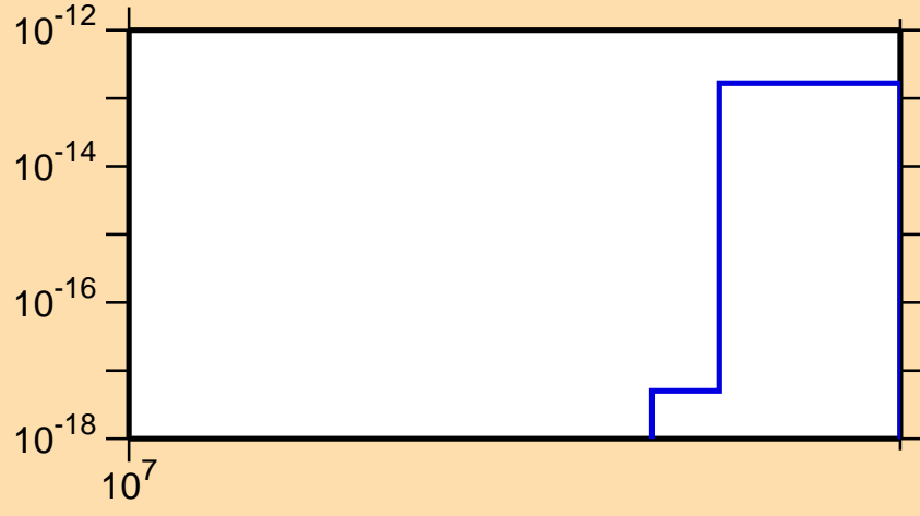
\sigma vs. E for ^{135}\text{Pr}(\text{mt 34})
