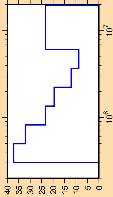
\Delta\sigma/\sigma vs. E for ^{135}\text{Pr}(n,n_4)
