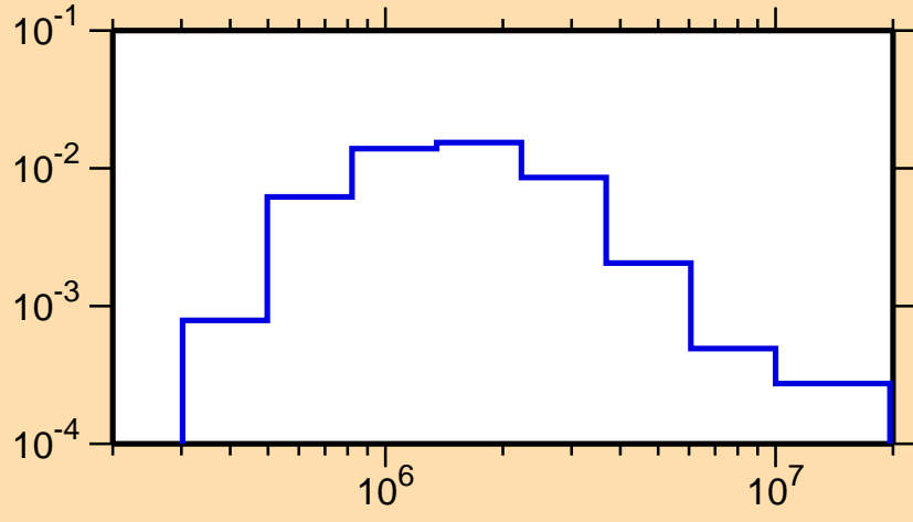
\sigma vs. E for ^{135}\text{Pr}(n,n_4)
