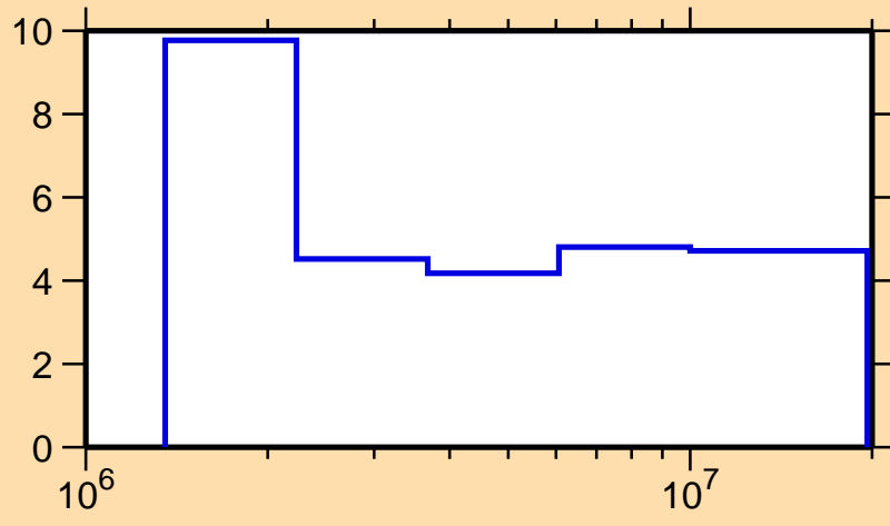
\Delta\sigma/\sigma vs. E for ^{135}\text{Pr}(n,n\text{onel.})
