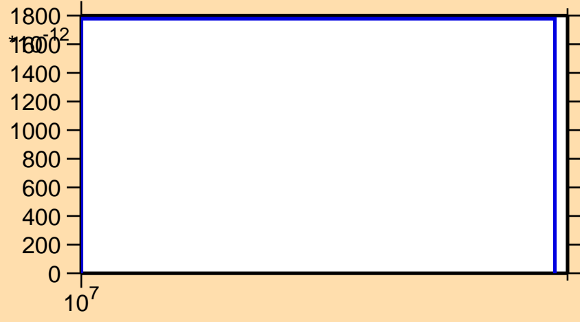
\sigma vs. E for ^{135}\text{Pr}(\text{mt } 45)
