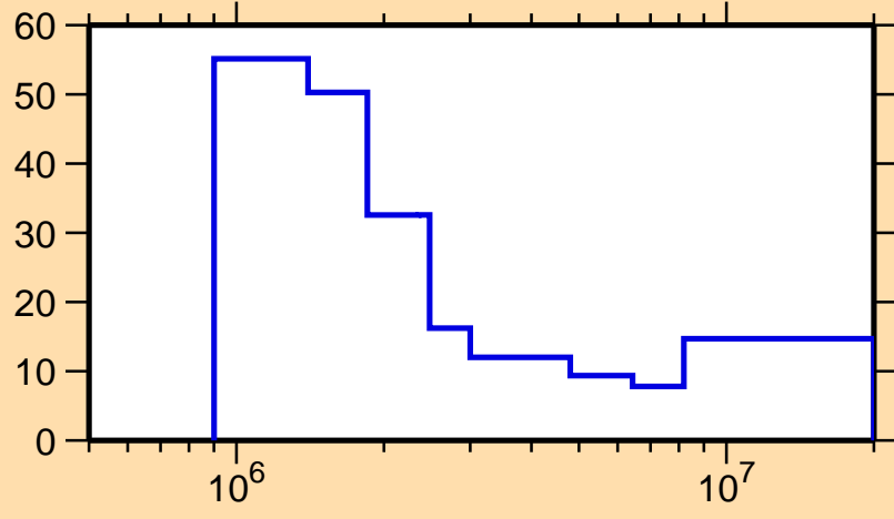
\Delta\sigma/\sigma vs. E for ^{135}\text{Pr}(n,n\text{cont.})
