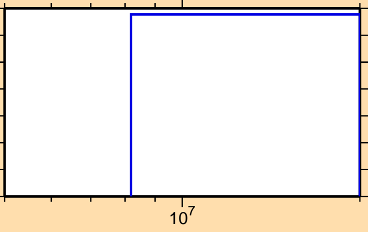
\sigma vs. E for ^{135}\text{Pr}(\text{mt } 34)
