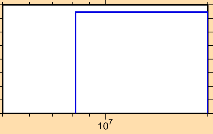
\sigma vs. E for ^{135}\text{Pr}(\text{mt } 11)
