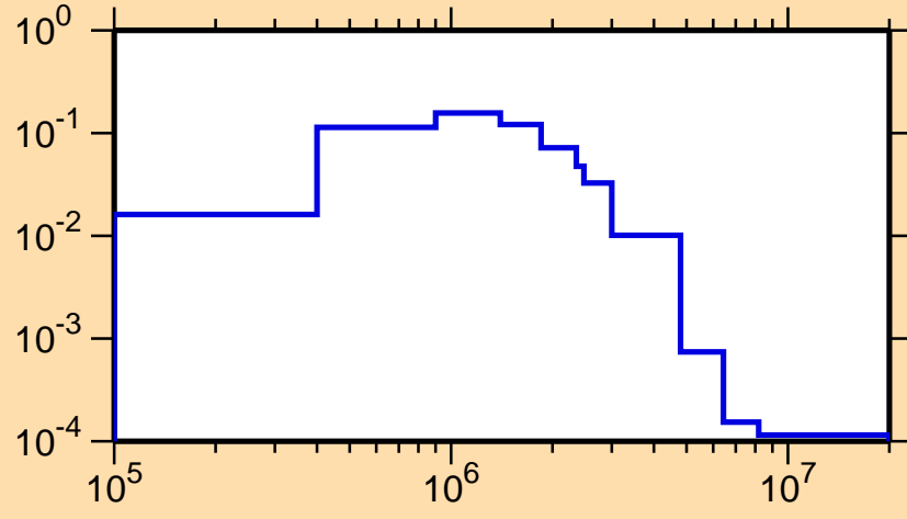
\sigma vs. E for ^{135}\text{Pr}(n,n_2)
