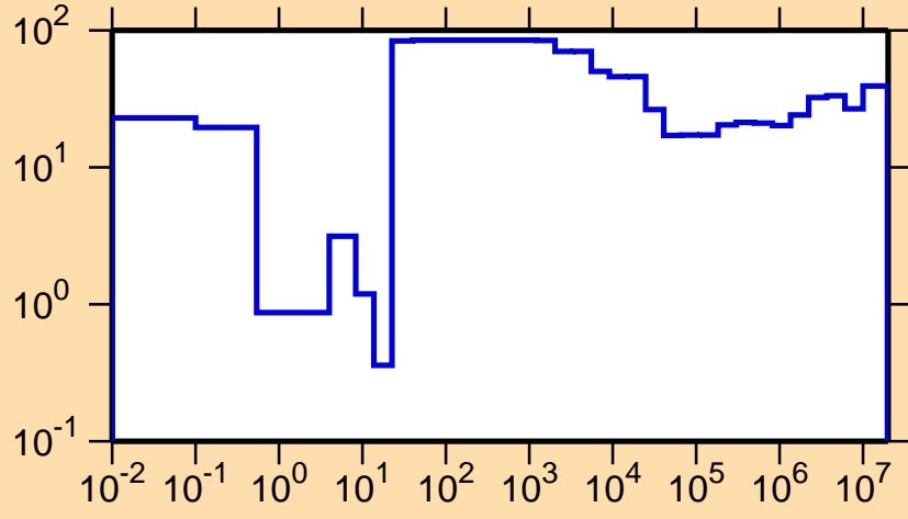
\Delta\sigma/\sigma vs. E for ^{136}\text{Pr}(n,\gamma)
