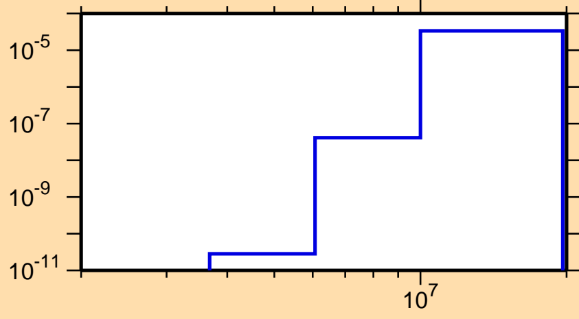
\sigma vs. E for ^{136}\text{Pr}(n,p\alpha)
