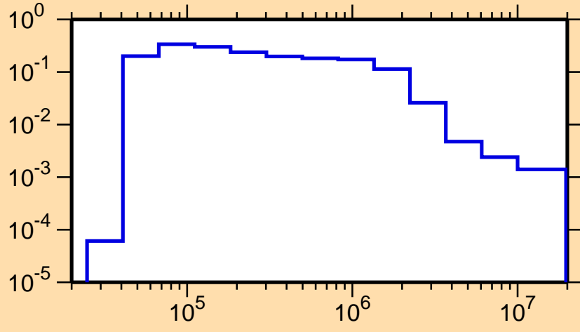
\sigma vs. E for ^{136}\text{Pr}(n,n_1)
