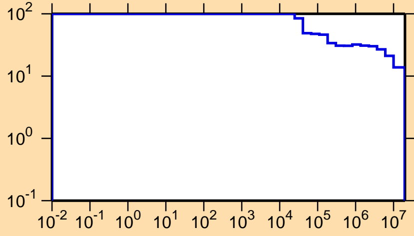
\Delta\sigma/\sigma vs. E for ^{136}\text{Pr}(n,p)
