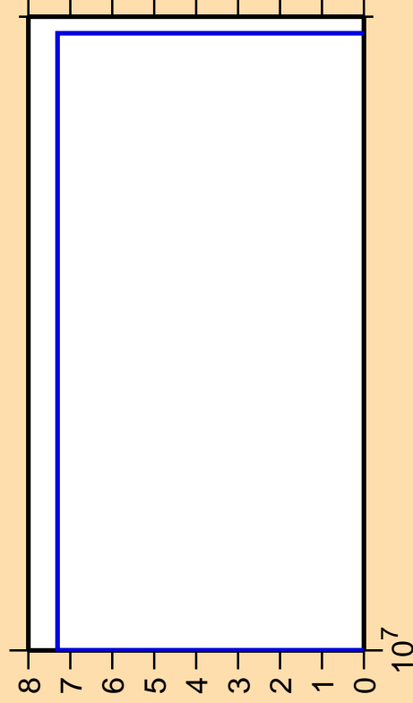
\Delta\sigma/\sigma vs. E for ^{136}\text{Pr}(n,\text{pt})
