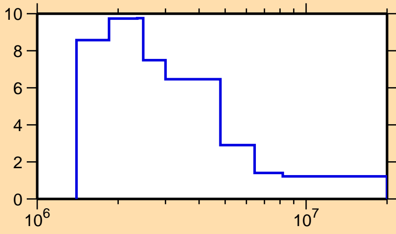
\Delta\sigma/\sigma vs. E for ^{136}\text{Pr}(n,\text{tot.})
