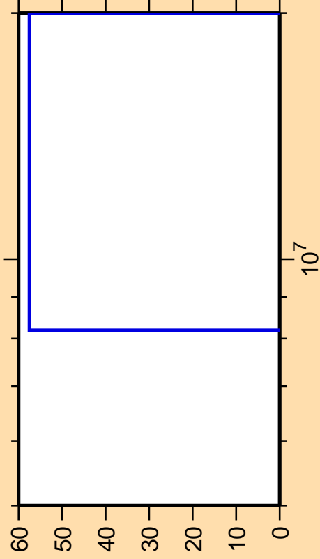
\Delta\sigma/\sigma vs. E for ^{136}\text{Pr}(n,pd)
