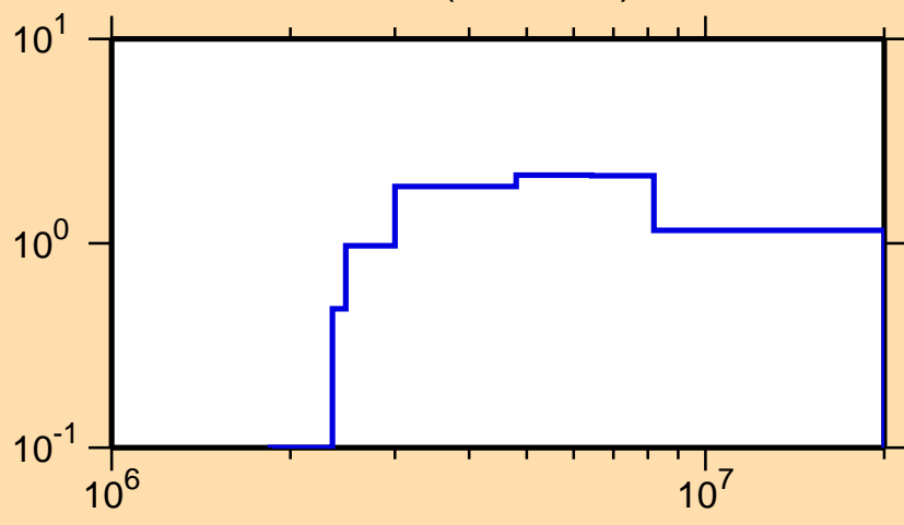
\sigma vs. E for ^{137}\text{Pr}(n,n\text{cont.})
