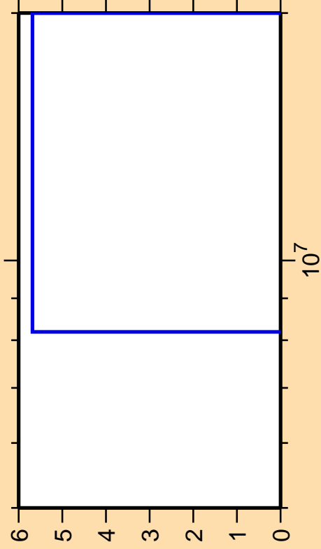
\Delta\sigma/\sigma vs. E for ^{137}\text{Pr}(n,2n)
