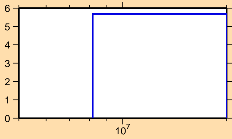
\Delta\sigma/\sigma vs. E for ^{137}\text{Pr}(n,2n)
