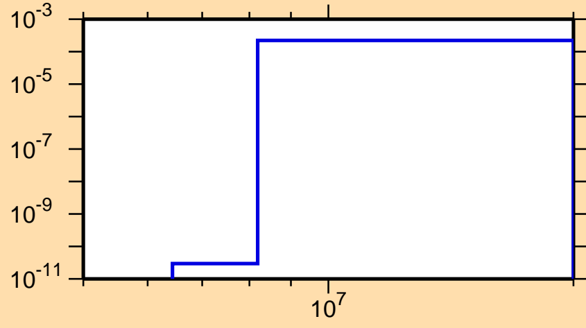
\sigma vs. E for ^{138}\text{Pr}(n,t)
