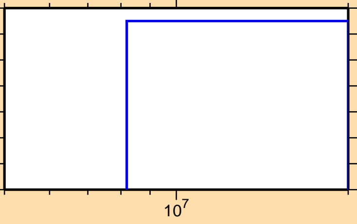
\sigma vs. E for ^{138}\text{Pr}(n,2n\alpha)
