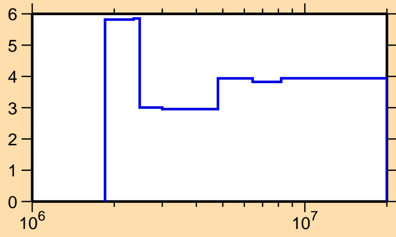
\Delta\sigma/\sigma vs. E for ^{138}\text{Pr}(n,\text{nonel.})
