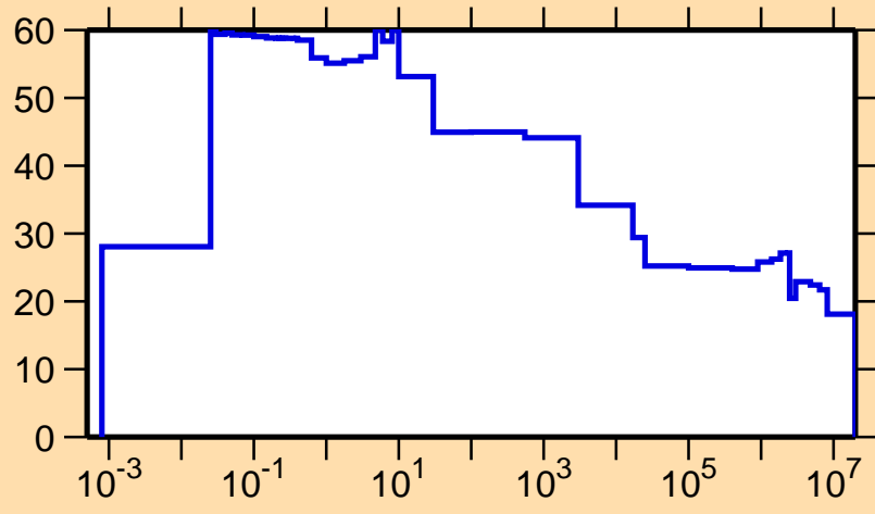
\Delta\sigma/\sigma vs. E for ^{138}\text{Pr}(n,p)
