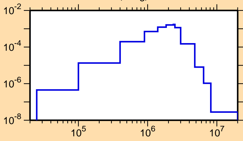
\sigma vs. E for ^{138}\text{Pr}(n,n_3)
