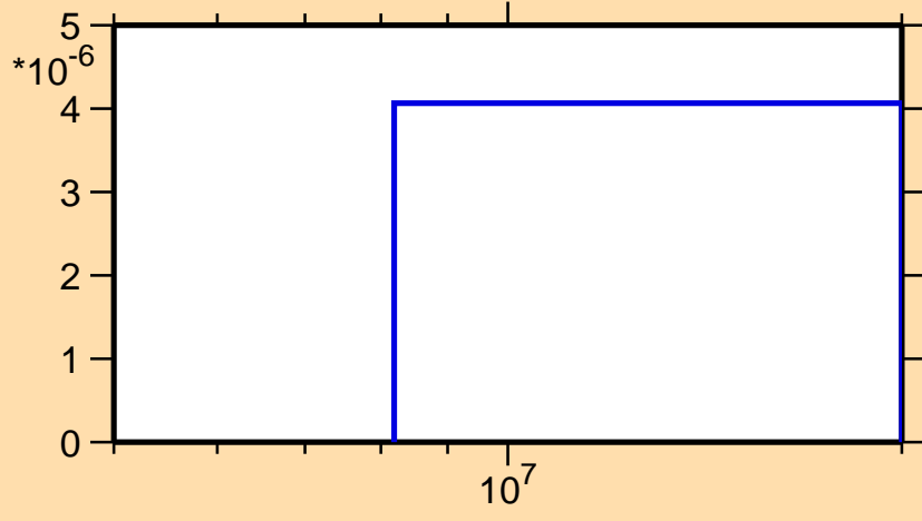
\sigma vs. E for ^{138}\text{Pr}(n,3n)
