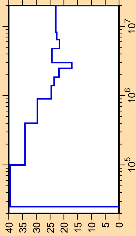
\Delta\sigma/\sigma vs. E for ^{138}\text{Pr}(n,n_3)
