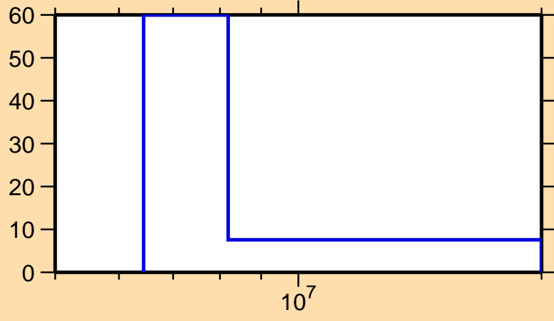
\Delta\sigma/\sigma vs. E for ^{138}\text{Pr}(n,2n)
