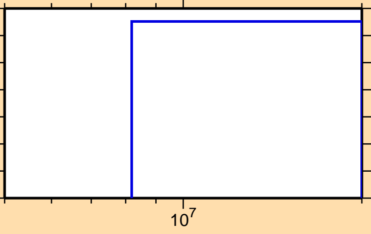
\sigma vs. E for ^{138}\text{Pr}(\text{mt117})
