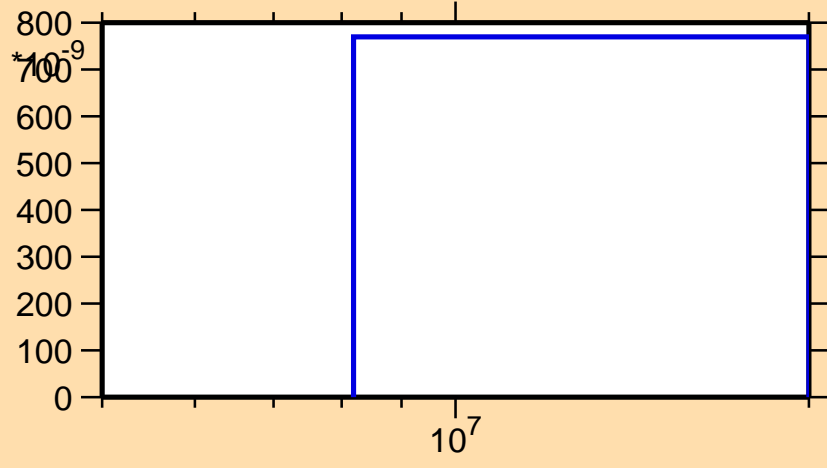
\sigma vs. E for ^{138}\text{Pr}(n,\text{nd})
