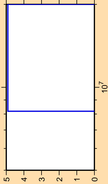
\Delta\sigma/\sigma vs. E for ^{138}\text{Pr}(n,\text{pd})
