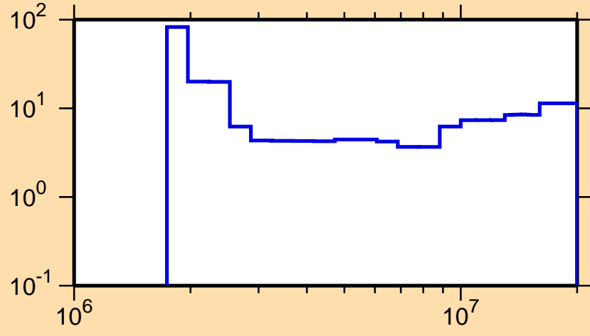
\Delta\sigma/\sigma vs. E for ^{139}\text{Pr}(n,n\text{cont.})
