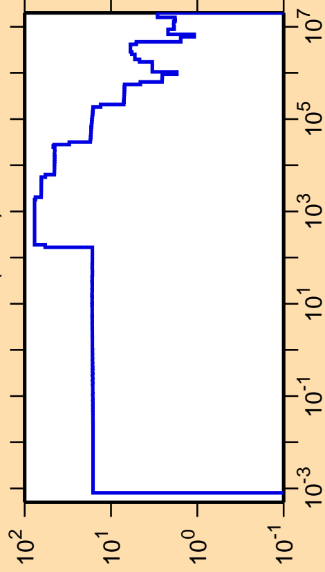
\Delta\sigma/\sigma vs. E for ^{139}\text{Pr}(n,\text{el.})
