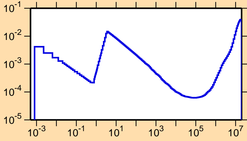
\sigma vs. E for ^{139}\text{Pr}(n,p)
