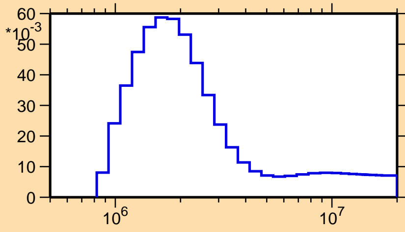
\sigma vs. E for ^{139}\text{Pr}(n,n_4)
