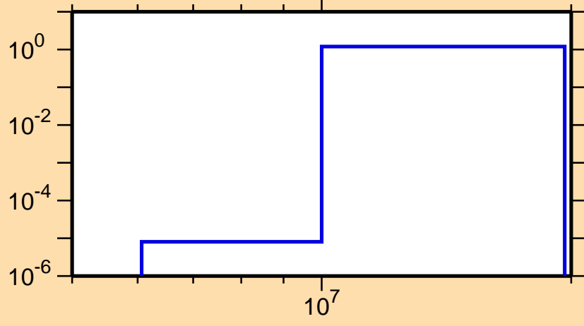
\sigma vs. E for ^{139}\text{Pr}(n,2n)
