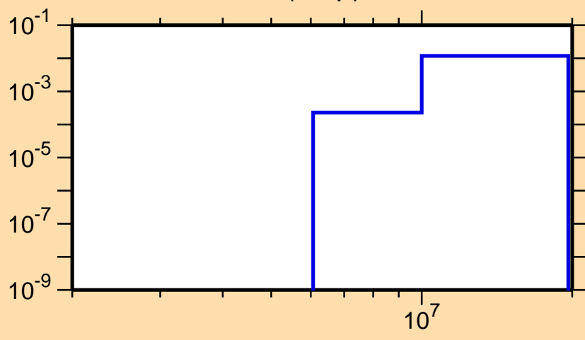
\sigma vs. E for ^{139}\text{Pr}(n,np)
