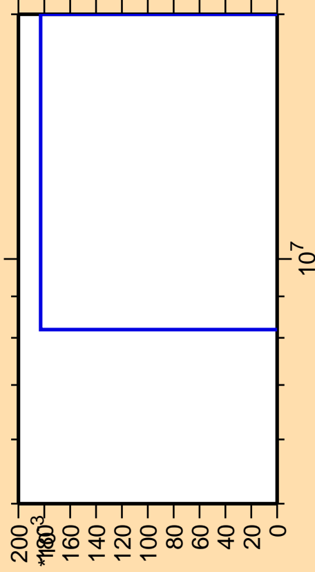
\Delta\sigma/\sigma vs. E for ^{139}\text{Pr}(\text{mt117})
