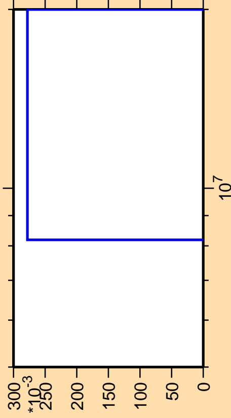
\Delta\sigma/\sigma vs. E for ^{139}\text{Pr}(\text{mt } 45)
