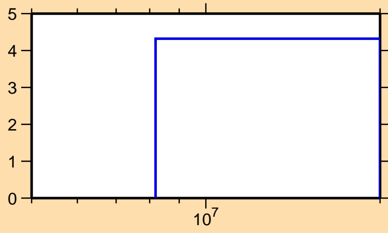
\Delta\sigma/\sigma vs. E for ^{139}\text{Pr}(n,\text{inel.})
