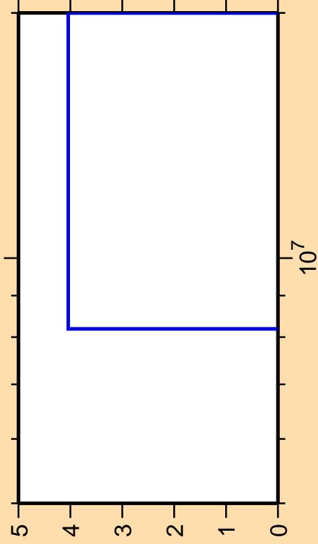
\Delta\sigma/\sigma vs. E for ^{139}\text{Pr}(n,2n)
