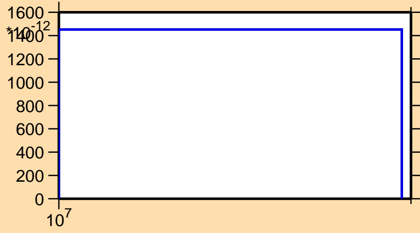
\sigma vs. E for ^{140}\text{Pr}(n,2n\alpha)
