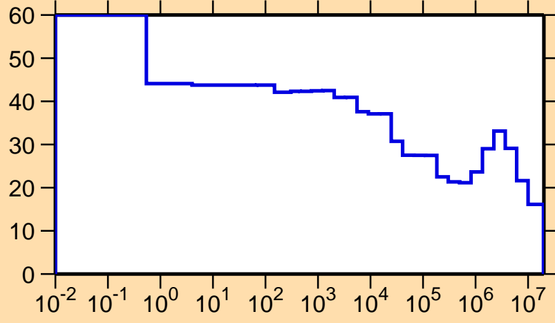
\Delta\sigma/\sigma vs. E for ^{140}\text{Pr}(n,p)
