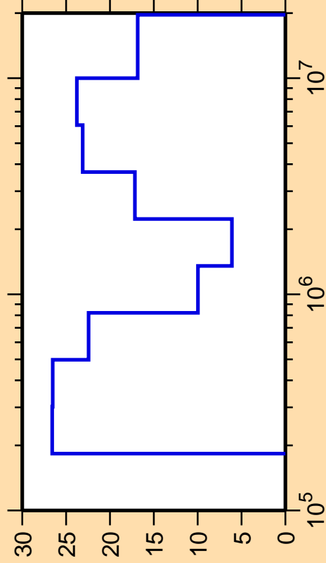
\Delta\sigma/\sigma vs. E for ^{140}\text{Pr}(n,n_4)
