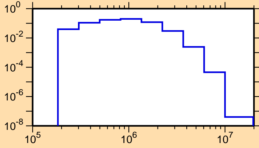
\sigma vs. E for ^{140}\text{Pr}(n,n_4)
