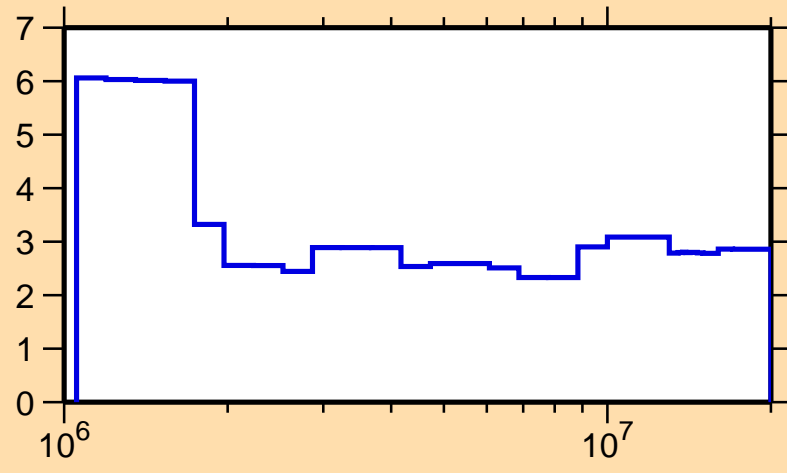
\Delta\sigma/\sigma vs. E for ^{142}\text{Pr}(n,n\text{oncl.})
