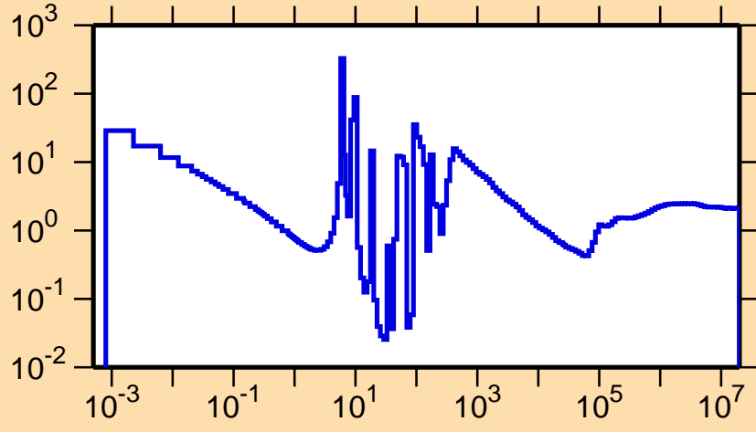
\sigma vs. E for ^{142}\text{Pr}(n,\text{nonel.})
