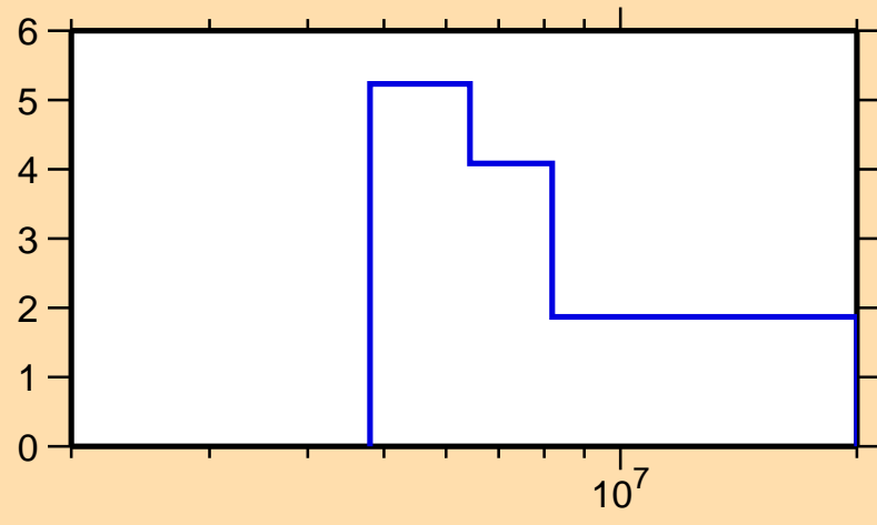
\Delta\sigma/\sigma vs. E for ^{142}\text{Pr}(n,2n)
