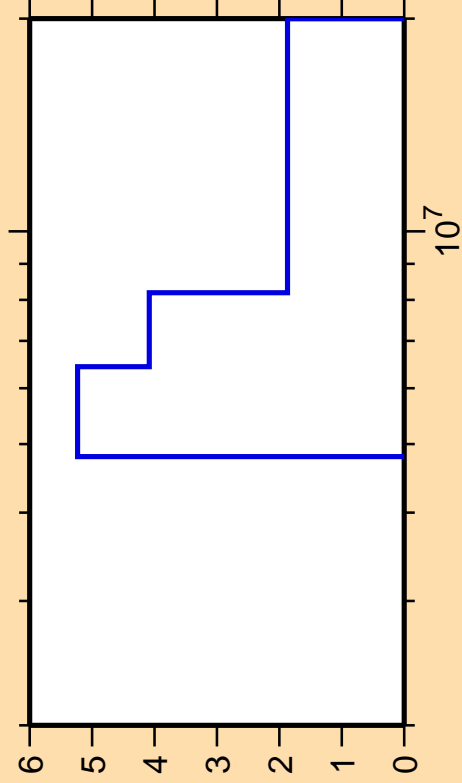
\Delta\sigma/\sigma vs. E for ^{142}\text{Pr}(n,2n)
