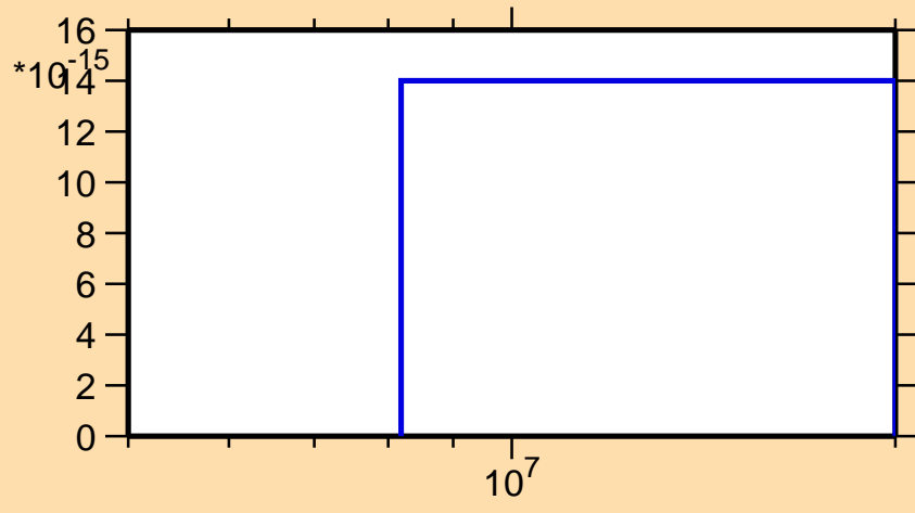
\sigma vs. E for ^{142}\text{Pr}(\text{mt117})
