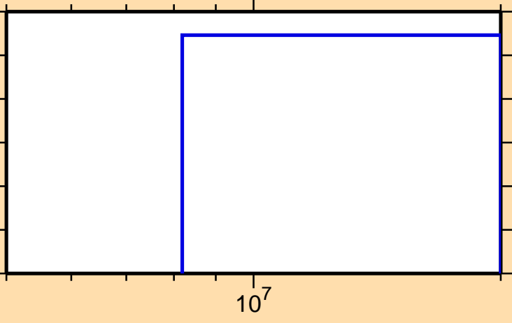
\sigma vs. E for ^{142}\text{Pr}(n,\text{He3})
