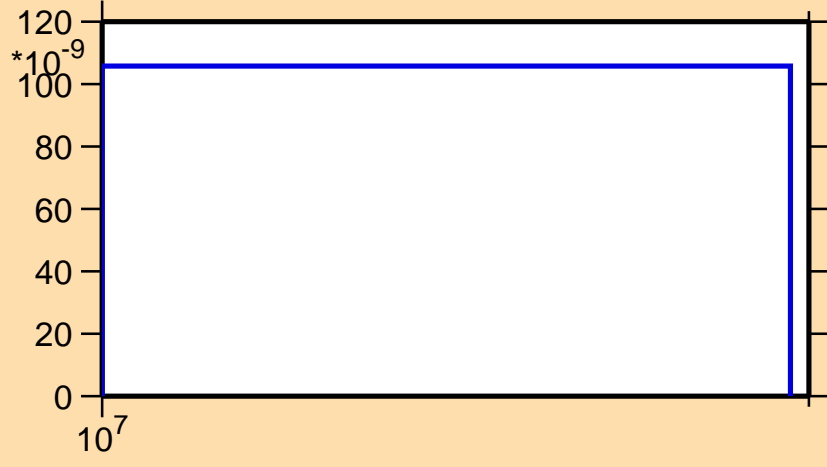
\sigma vs. E for ^{143}\text{Pr}(n,2np)
