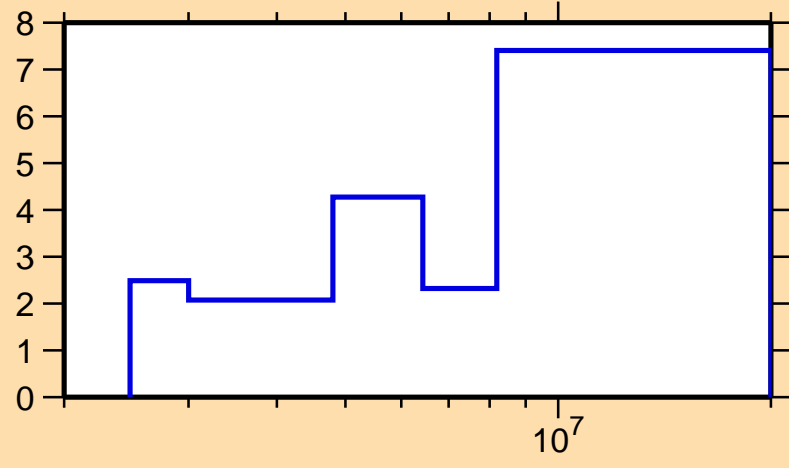
\Delta\sigma/\sigma vs. E for ^{143}\text{Pr}(n,\text{inel.})
