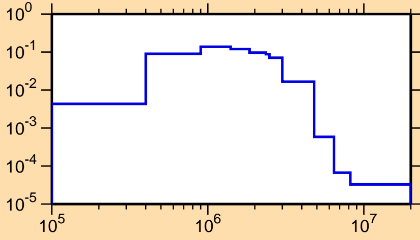
\sigma vs. E for ^{143}\text{Pr}(n,n_2)
