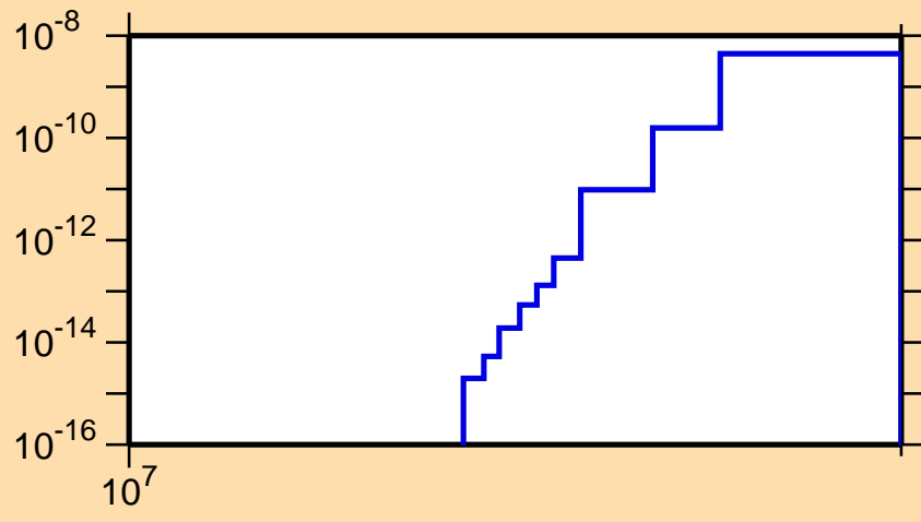
\sigma vs. E for ^{144}\text{Pr}(n,\text{He3})
