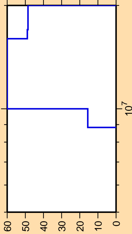
\Delta\sigma/\sigma vs. E for ^{144}\text{Pr}(n,2n\alpha)
