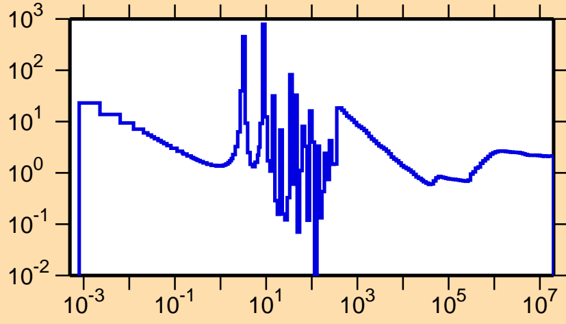
\sigma vs. E for ^{144}\text{Pr}(n,\text{nonel.})
