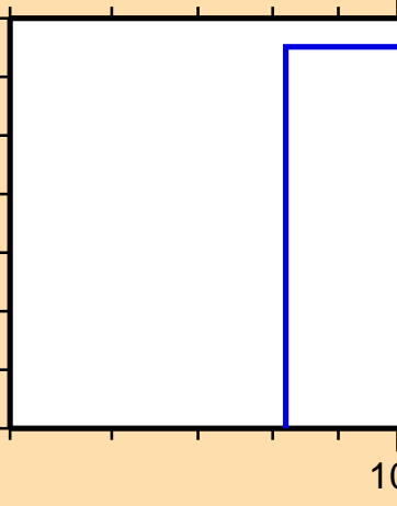
\sigma vs. E for ^{144}\text{Pr}(\text{mt } 45)
