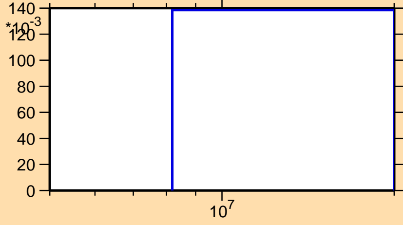
\sigma vs. E for ^{144}\text{Pr}(n,3n)
