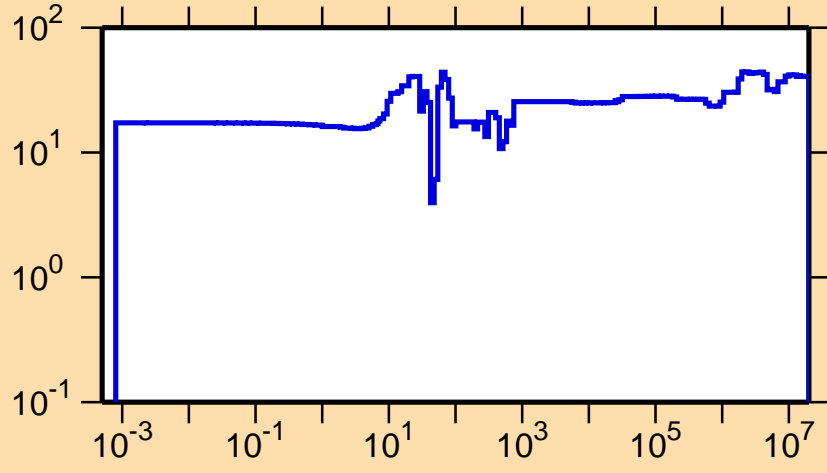
\Delta\sigma/\sigma vs. E for ^{145}\text{Pr}(n,\gamma)
