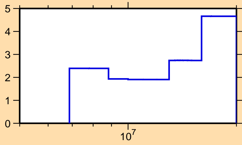
\Delta\sigma/\sigma vs. E for ^{145}\text{Pr}(n,\text{el.})
