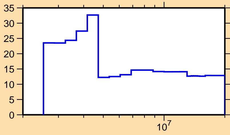
\Delta\sigma/\sigma vs. E for ^{145}\text{Pr}(n,n_1)
