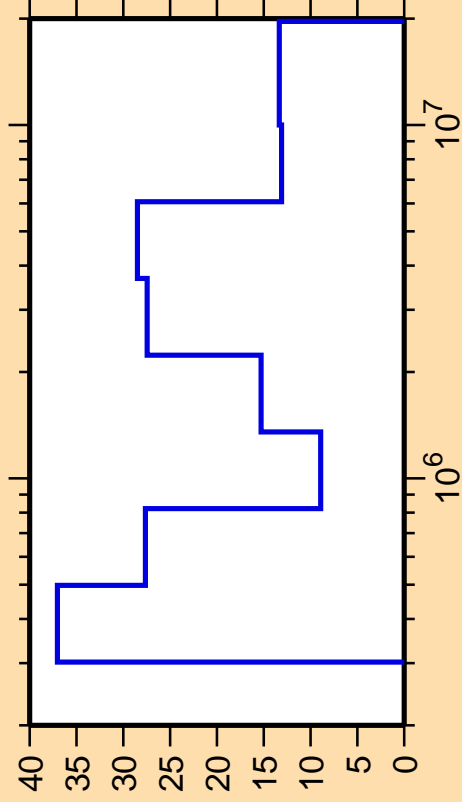
\Delta\sigma/\sigma vs. E for ^{145}\text{Pr}(n,n_3)
