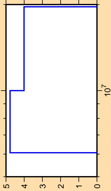
\Delta\sigma/\sigma vs. E for ^{145}\text{Pr}(n,2n)
