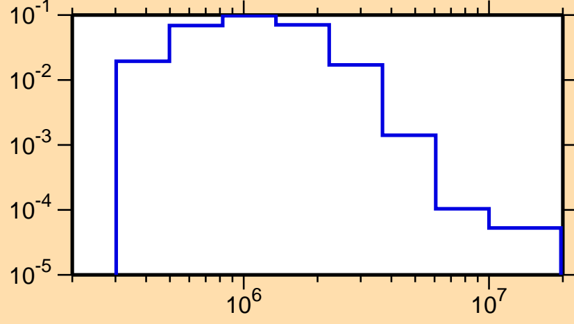
\sigma vs. E for ^{145}\text{Pr}(n,n_3)
