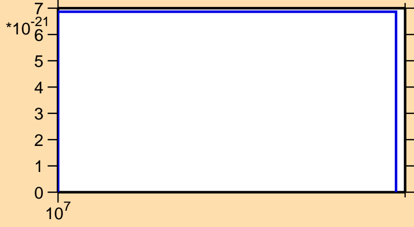
\sigma vs. E for ^{145}\text{Pr}(\text{mt } 42)
