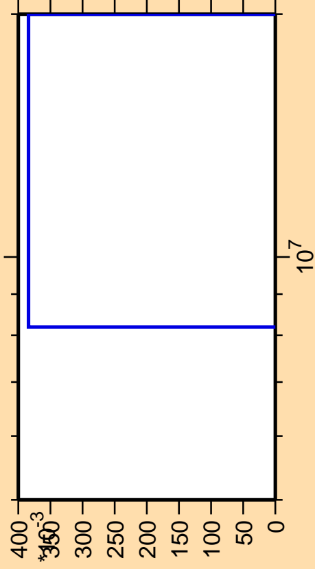
\Delta\sigma/\sigma vs. E for ^{145}\text{Pr}(n,p\alpha)
