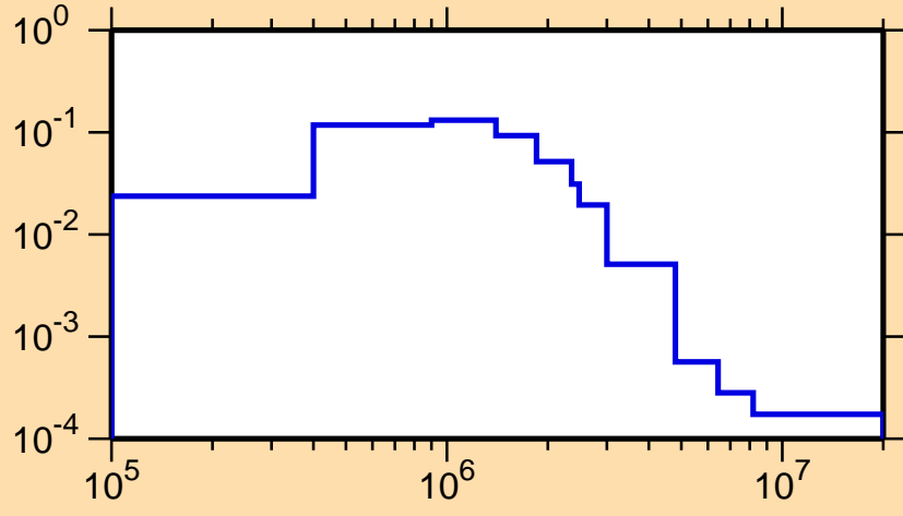
\sigma vs. E for ^{145}\text{Pr}(n,n_2)
