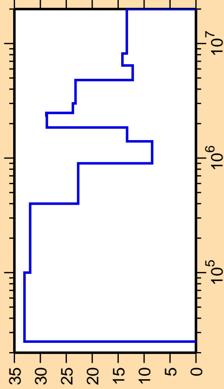
\Delta\sigma/\sigma vs. E for ^{145}\text{Pr}(n,n_1)
