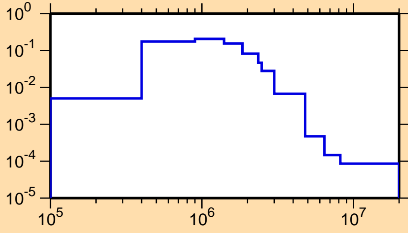
\sigma vs. E for ^{145}\text{Pr}(n,n_4)
