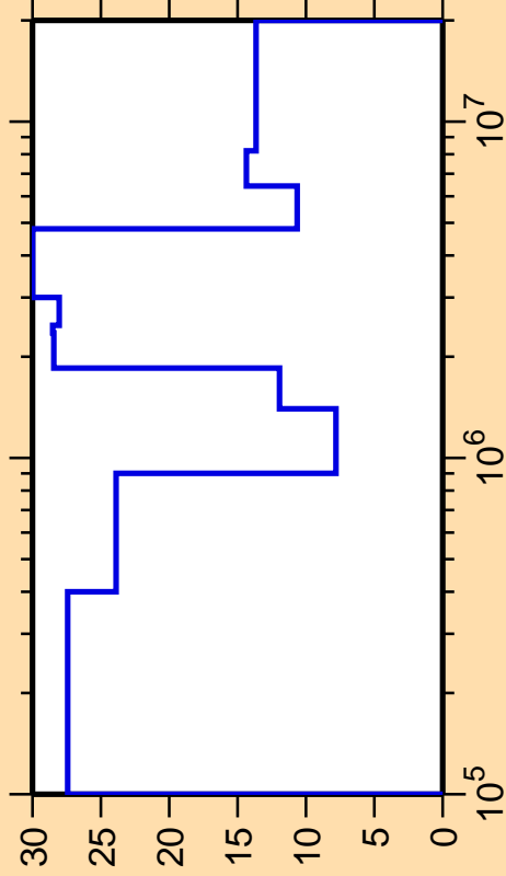
\Delta\sigma/\sigma vs. E for ^{145}\text{Pr}(n,n_4)
