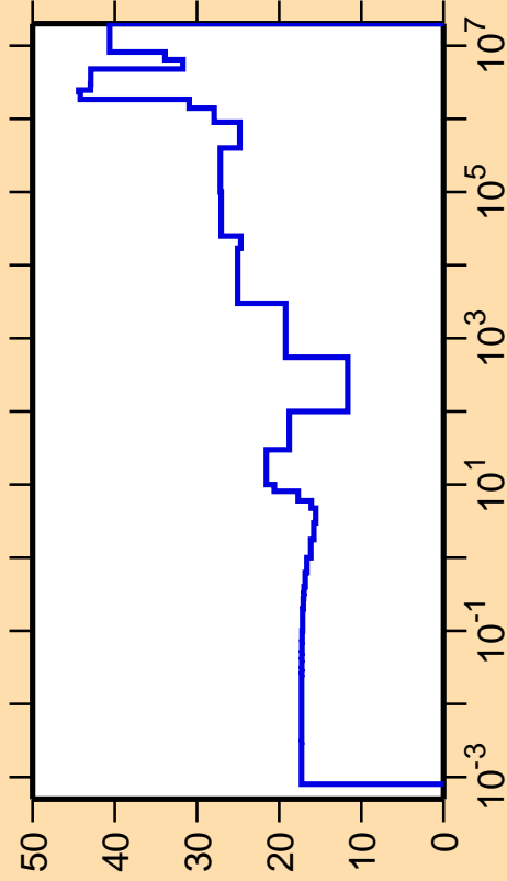
\Delta\sigma/\sigma vs. E for ^{145}\text{Pr}(n,\gamma)
