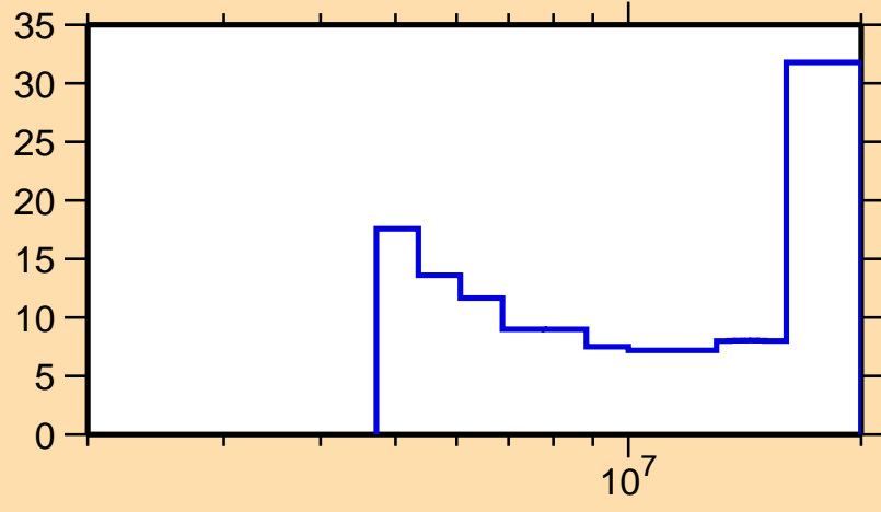
\Delta\sigma/\sigma vs. E for ^{146}\text{Pr}(n,2n)
