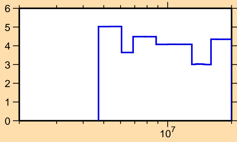
\Delta\sigma/\sigma vs. E for ^{146}\text{Pr}(n,\text{el.})
