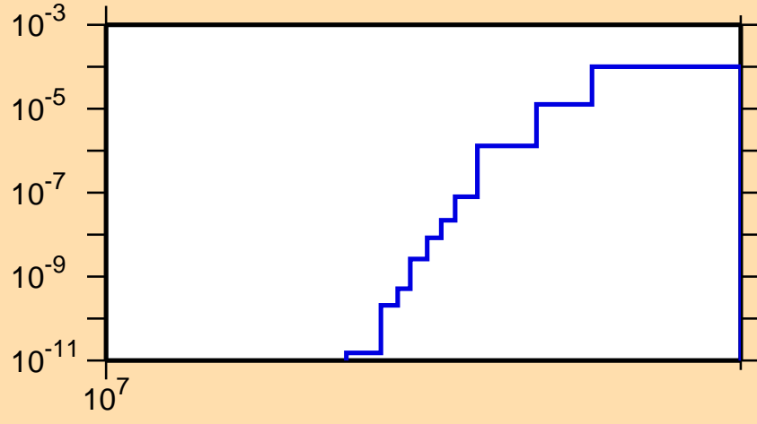
\sigma vs. E for ^{146}\text{Pr}(n,nt)
