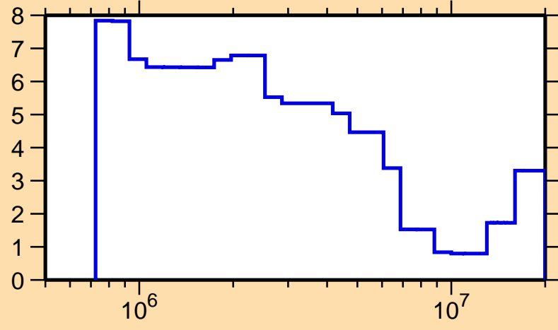
\Delta\sigma/\sigma vs. E for ^{146}\text{Pr}(n,\text{tot.})
