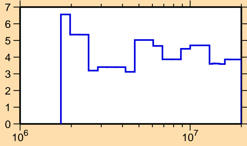
\Delta\sigma/\sigma vs. E for ^{146}\text{Pr}(n,\text{nonel.})
