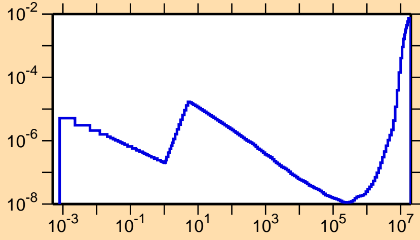
\sigma vs. E for ^{146}\text{Pr}(n,\alpha)
