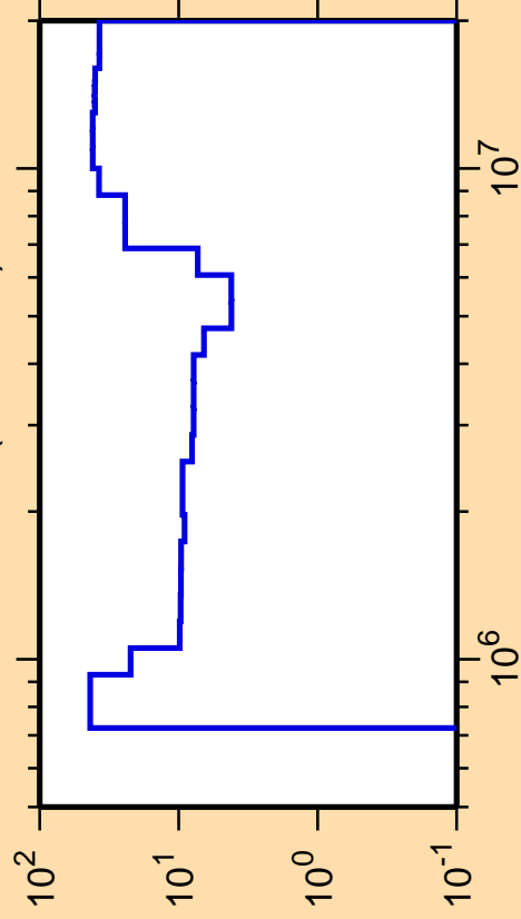
\Delta\sigma/\sigma vs. E for ^{146}\text{Pr}(n,n\text{cont.})
