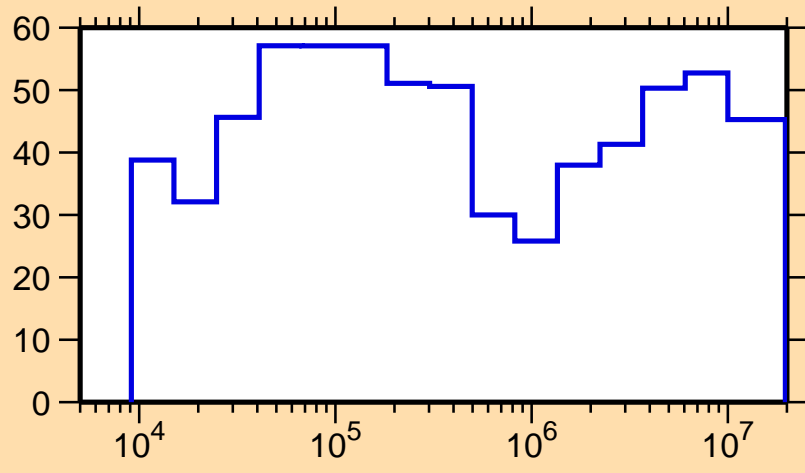
\Delta\sigma/\sigma vs. E for ^{146}\text{Pr}(n,n_1)
