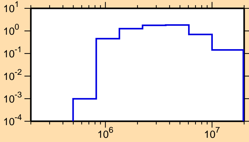
\sigma vs. E for ^{146}\text{Pr}(n,n\text{cont.})
