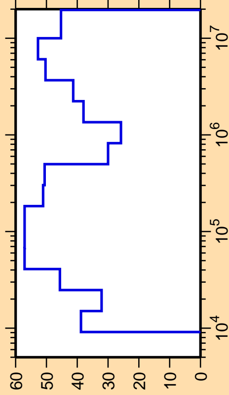
\Delta\sigma/\sigma vs. E for ^{146}\text{Pr}(n,n_1)
