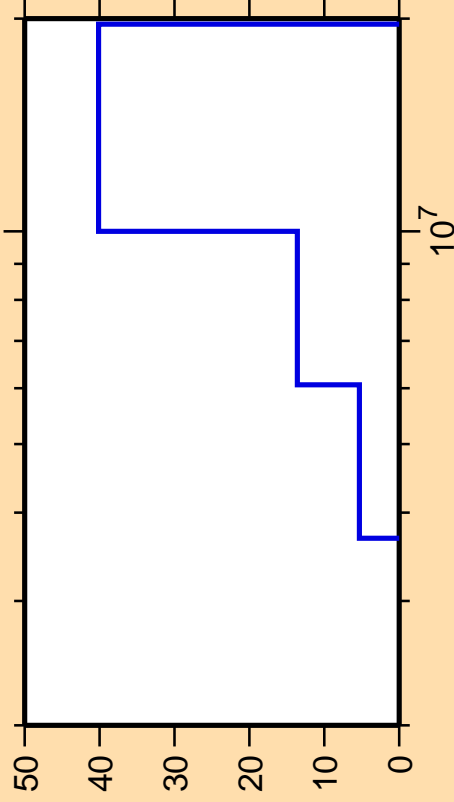
\Delta\sigma/\sigma vs. E for ^{146}\text{Pr}(n,n\text{cont.})
