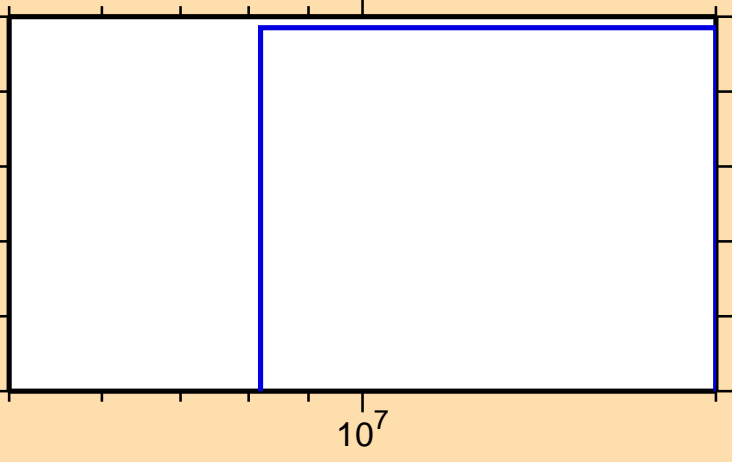
\sigma vs. E for ^{146}\text{Pr}(n,2n\alpha)
