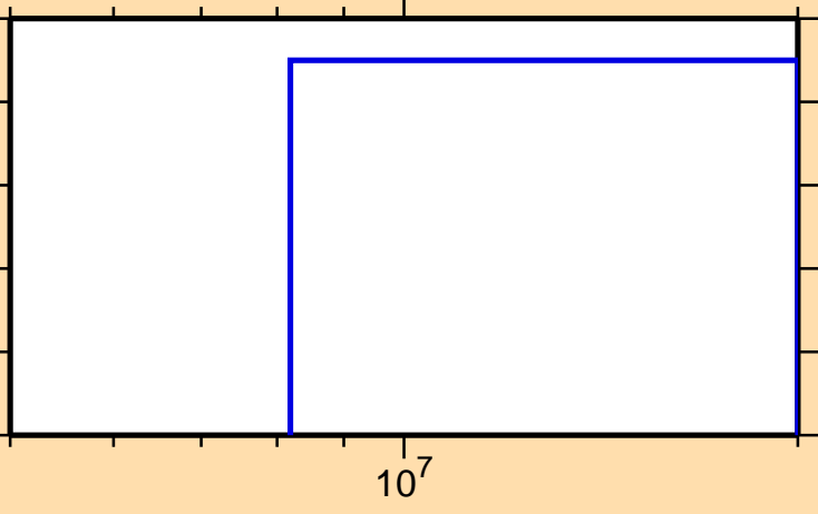
\sigma vs. E for ^{146}\text{Pr}(n,3n\alpha)
