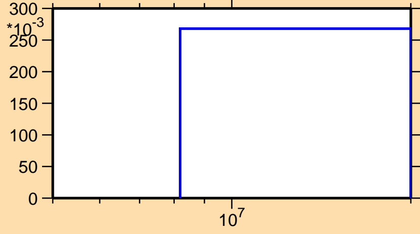
\sigma vs. E for ^{146}\text{Pr}(n,3n)
