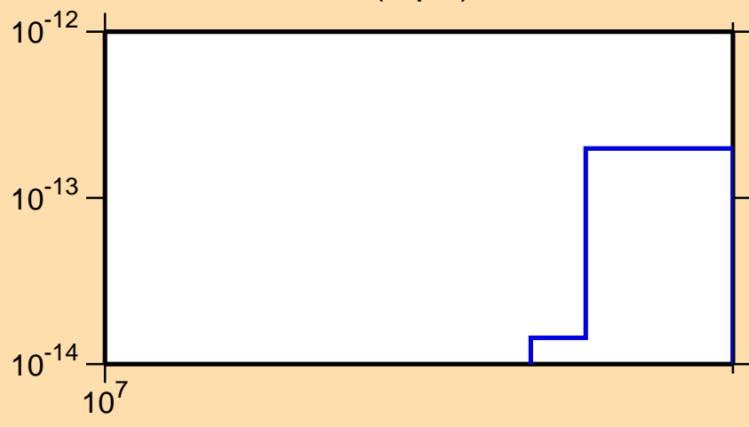
\sigma vs. E for ^{147}\text{Pr}(n,p\alpha)
