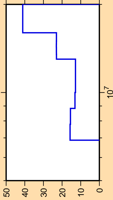
\Delta\sigma/\sigma vs. E for ^{147}\text{Pr}(n,2n)
