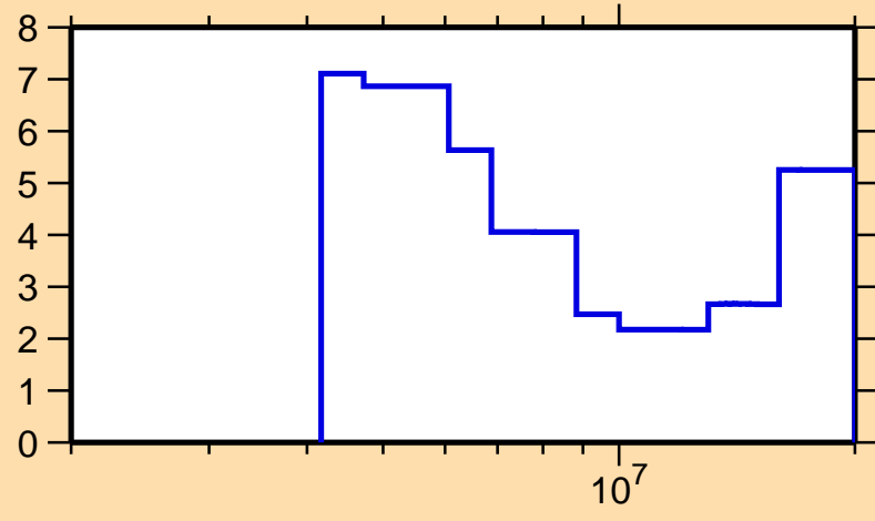
\Delta\sigma/\sigma vs. E for ^{147}\text{Pr}(n,\text{tot.})
