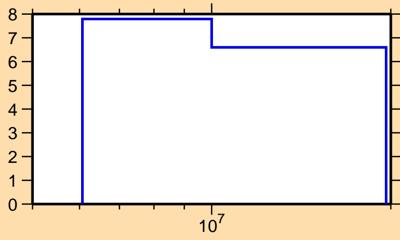
\Delta\sigma/\sigma vs. E for ^{147}\text{Pr}(n,\text{el.})
