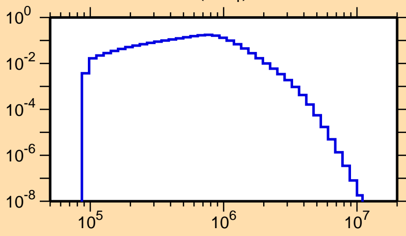
\sigma vs. E for ^{148}\text{Pr}(n,n_1)
