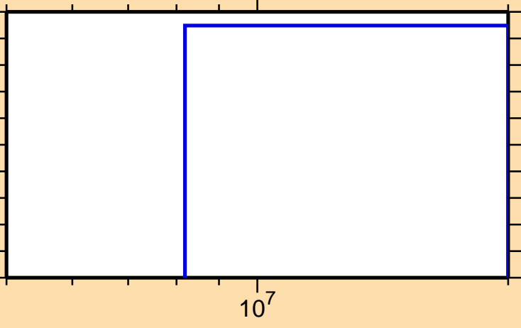
\sigma vs. E for ^{148}\text{Pr}(n,3n\alpha)
