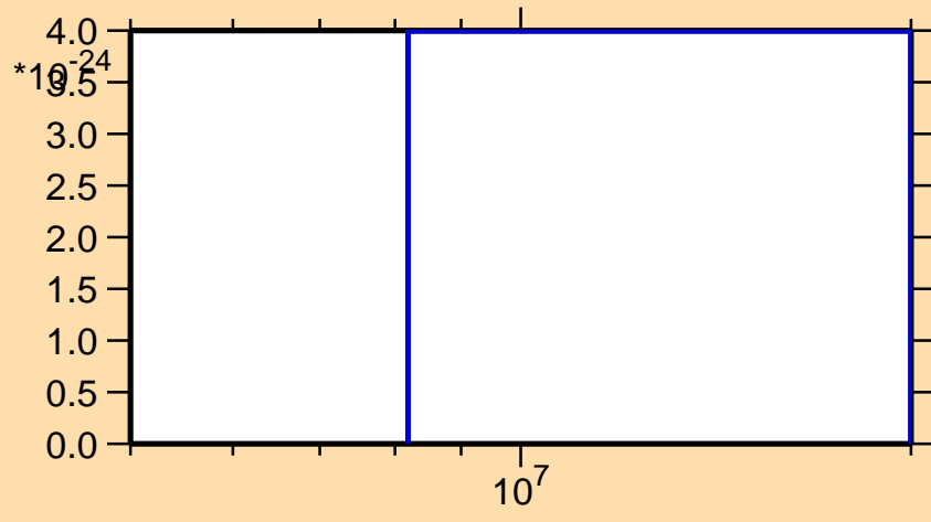
\sigma vs. E for ^{148}\text{Pr}(\text{mt } 42)
