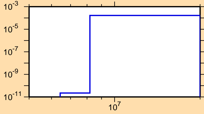
\sigma vs. E for ^{148}\text{Pr}(n,n\alpha)
