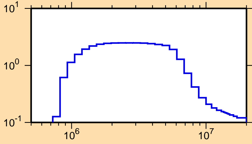
\sigma vs. E for ^{148}\text{Pr}(n,n\text{cont.})
