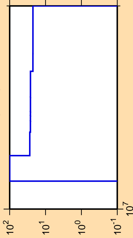
\Delta\sigma/\sigma vs. E for ^{148}\text{Pr}(n,3n)
