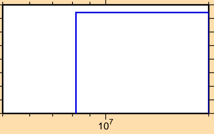
\sigma vs. E for ^{150}\text{Pr}(n,2n\alpha)
