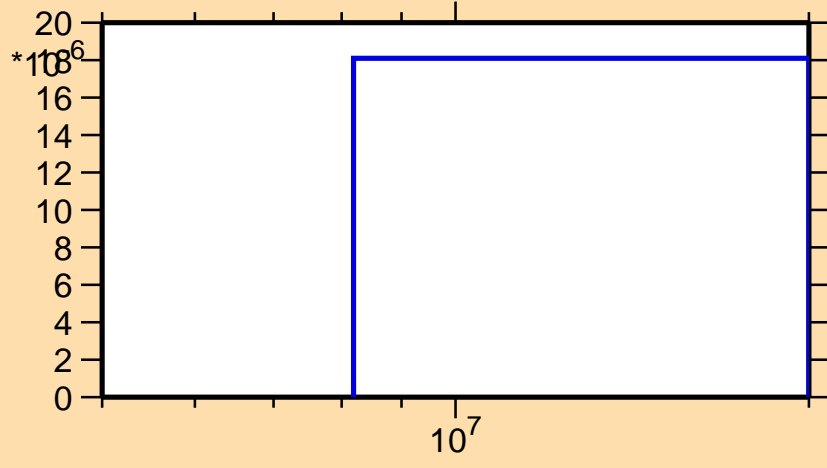
\sigma vs. E for ^{150}\text{Pr}(n,n\alpha)
