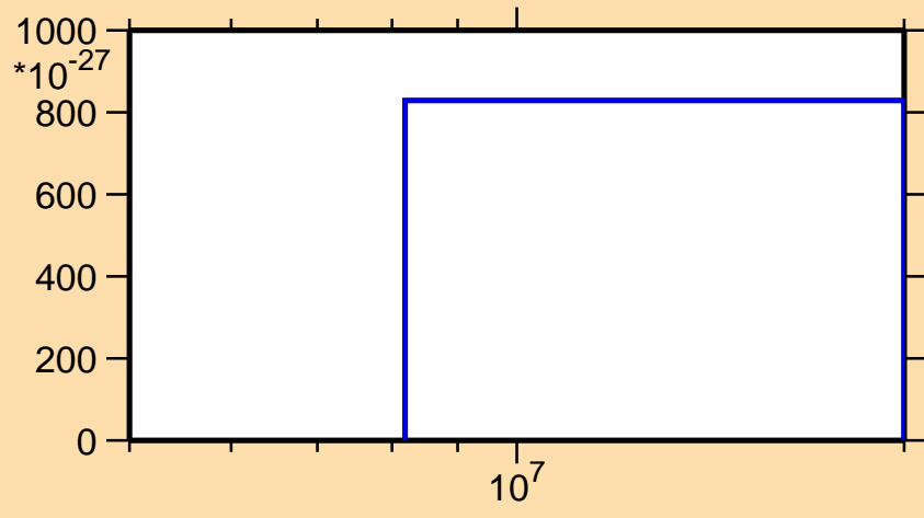
\sigma vs. E for ^{150}\text{Pr}(\text{mt } 42)
